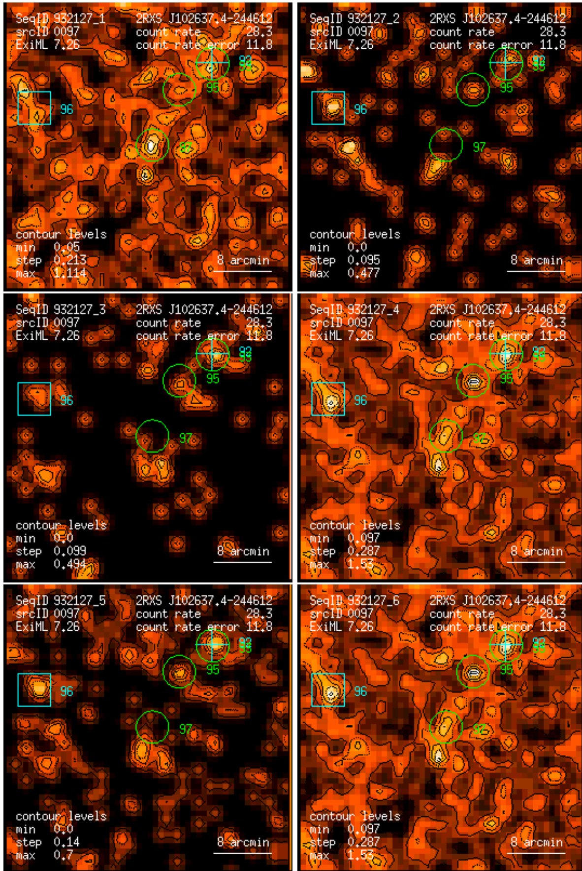
Figure 97: RASS 932127: detection 0097: band rate images, Gaussian filter: (1) PSPC channels 11 – 41, (2) 52 – 90, (3) 91 – 201, (4) 11 – 235, (5) 52 – 201, (6) 11 – 201. Broad band rates in counts/ks. Band rate contour levels in counts/ks/arcmin 2 .
