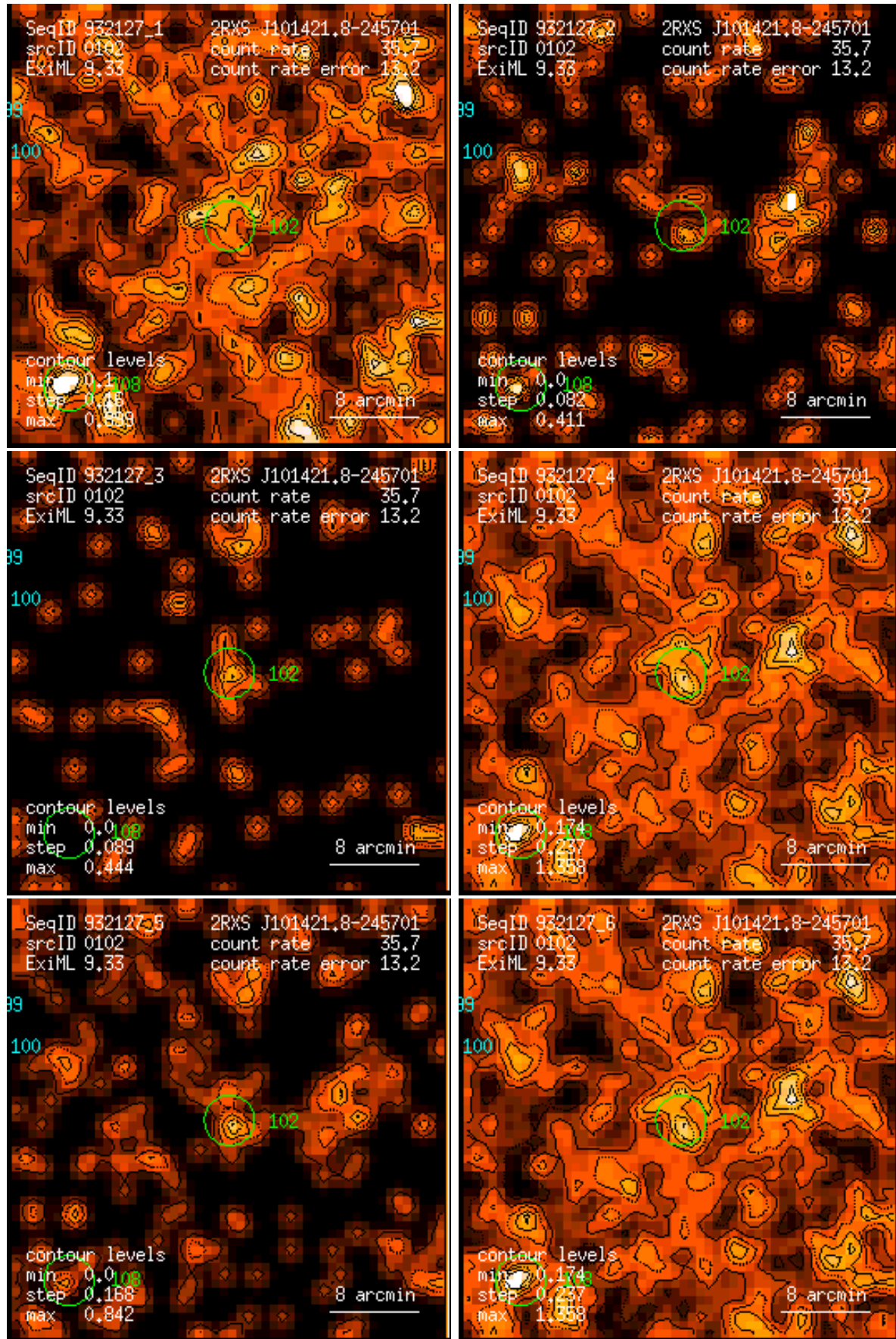
Figure 102: RASS 932127: detection 0102: band rate images, Gaussian filter: (1) PSPC channels 11 – 41, (2) 52 – 90, (3) 91 – 201, (4) 11 – 235, (5) 52 – 201, (6) 11 – 201. Broad band rates in counts/ks. Band rate contour levels in counts/ks/arcmin 2 .
