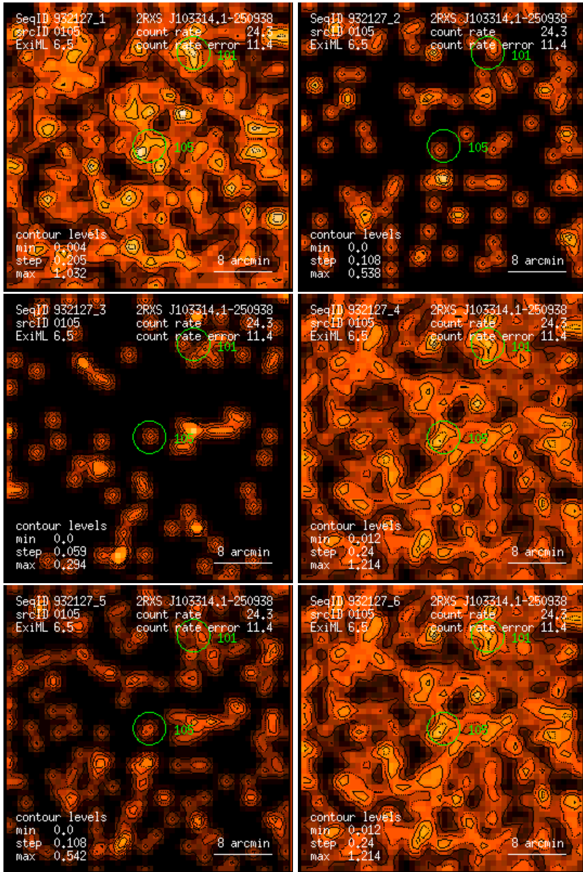
Figure 105: RASS 932127: detection 0105: band rate images, Gaussian filter: (1) PSPC channels 11 – 41, (2) 52 – 90, (3) 91 – 201, (4) 11 – 235, (5) 52 – 201, (6) 11 – 201. Broad band rates in counts/ks. Band rate contour levels in counts/ks/arcmin 2 .
