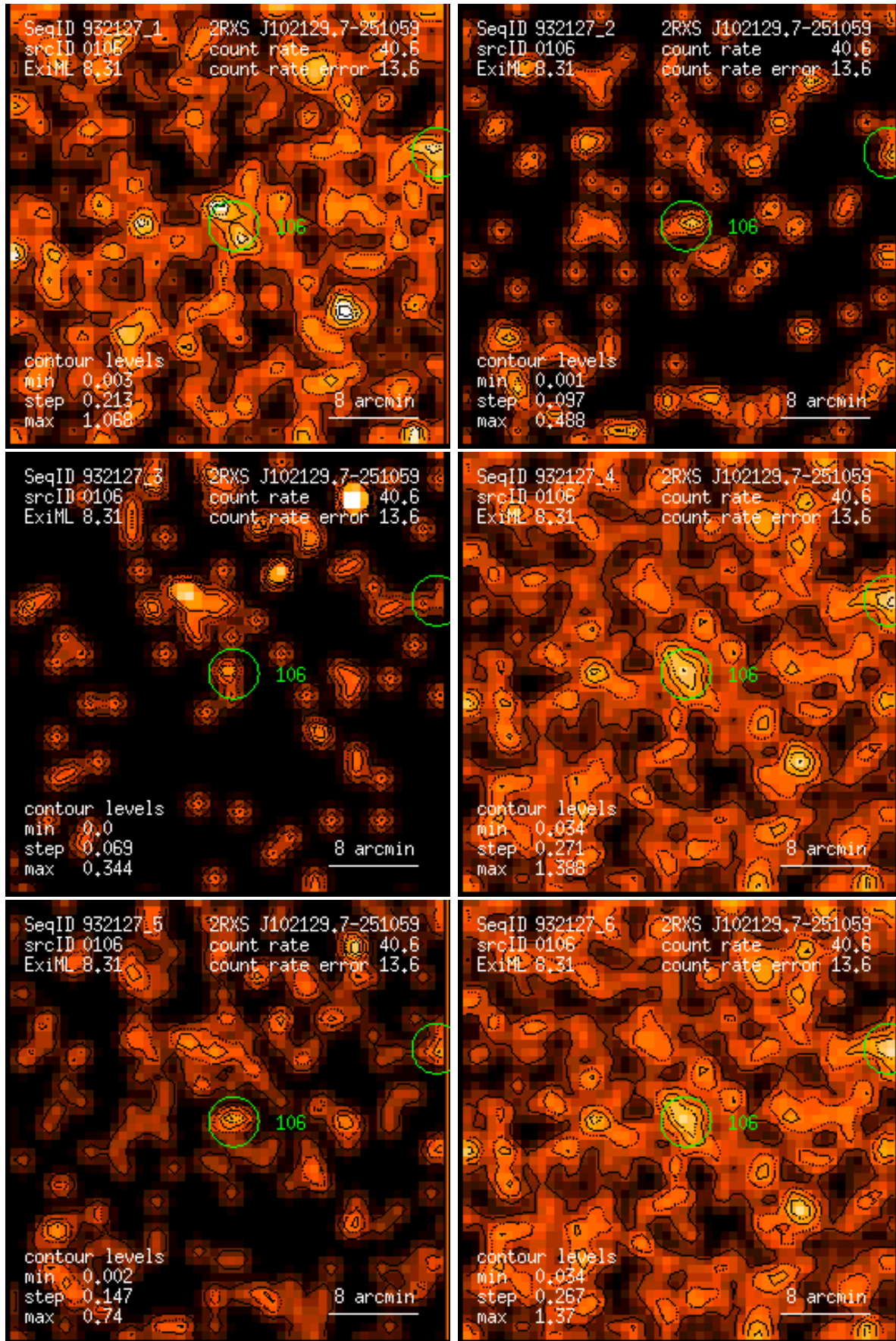
Figure 106: RASS 932127: detection 0106: band rate images, Gaussian filter: (1) PSPC channels 11 – 41, (2) 52 – 90, (3) 91 – 201, (4) 11 – 235, (5) 52 – 201, (6) 11 – 201. Broad band rates in counts/ks. Band rate contour levels in counts/ks/arcmin 2 .
