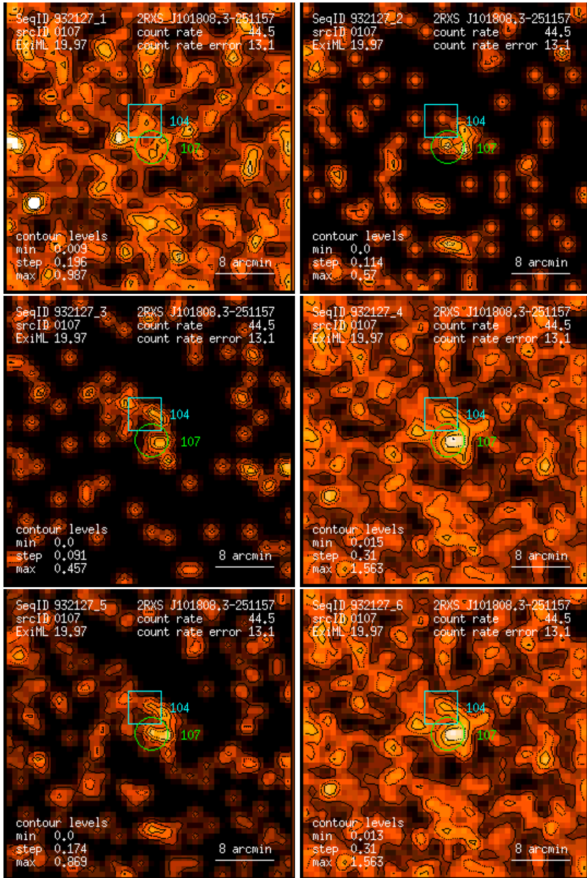
Figure 107: RASS 932127: detection 0107: band rate images, Gaussian filter: (1) PSPC channels 11 – 41, (2) 52 – 90, (3) 91 – 201, (4) 11 – 235, (5) 52 – 201, (6) 11 – 201. Broad band rates in counts/ks. Band rate contour levels in counts/ks/arcmin 2 .
