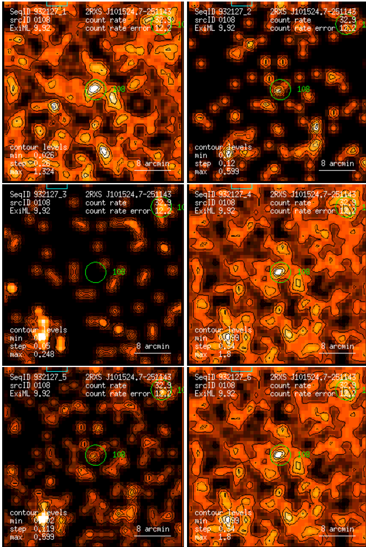
Figure 108: RASS 932127: detection 0108: band rate images, Gaussian filter: (1) PSPC channels 11 – 41, (2) 52 – 90, (3) 91 – 201, (4) 11 – 235, (5) 52 – 201, (6) 11 – 201. Broad band rates in counts/ks. Band rate contour levels in counts/ks/arcmin 2 .
