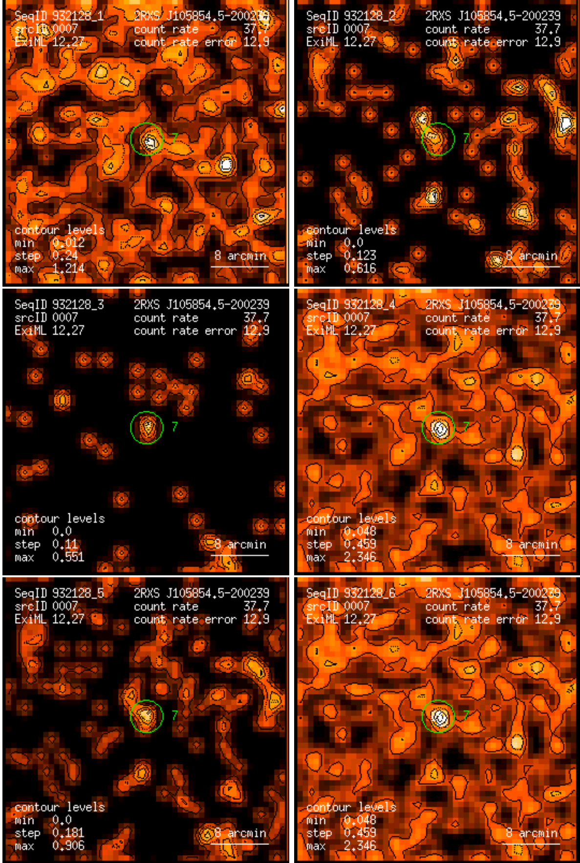
Figure 7: RASS 932128: detection 0007: band rate images, Gaussian filter: (1) PSPC channels 11 – 41, (2) 52 – 90, (3) 91 – 201, (4) 11 – 235, (5) 52 – 201, (6) 11 – 201. Broad band rates in counts/ks. Band rate contour levels in counts/ks/arcmin 2 .
