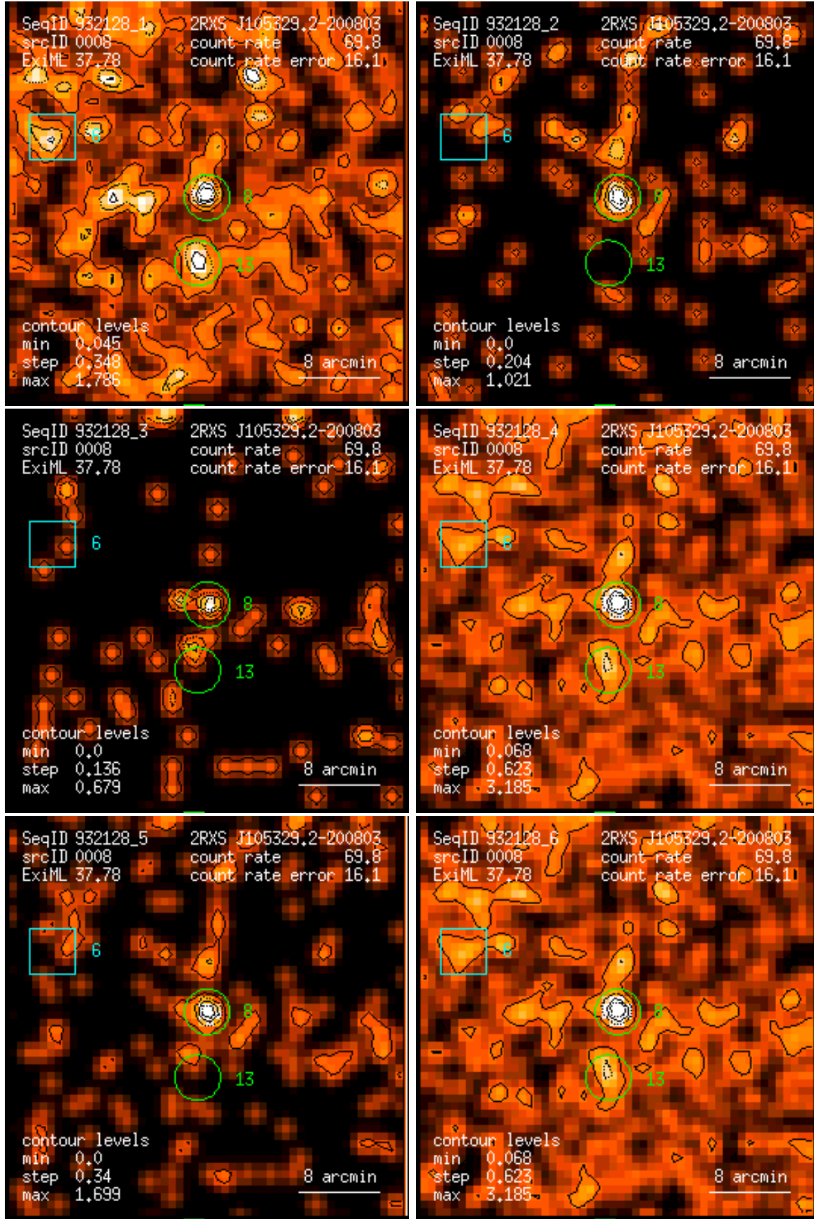
Figure 8: RASS 932128: detection 0008: band rate images, Gaussian filter: (1) PSPC channels 11 – 41, (2) 52 – 90, (3) 91 – 201, (4) 11 – 235, (5) 52 – 201, (6) 11 – 201. Broad band rates in counts/ks. Band rate contour levels in counts/ks/arcmin 2 .
