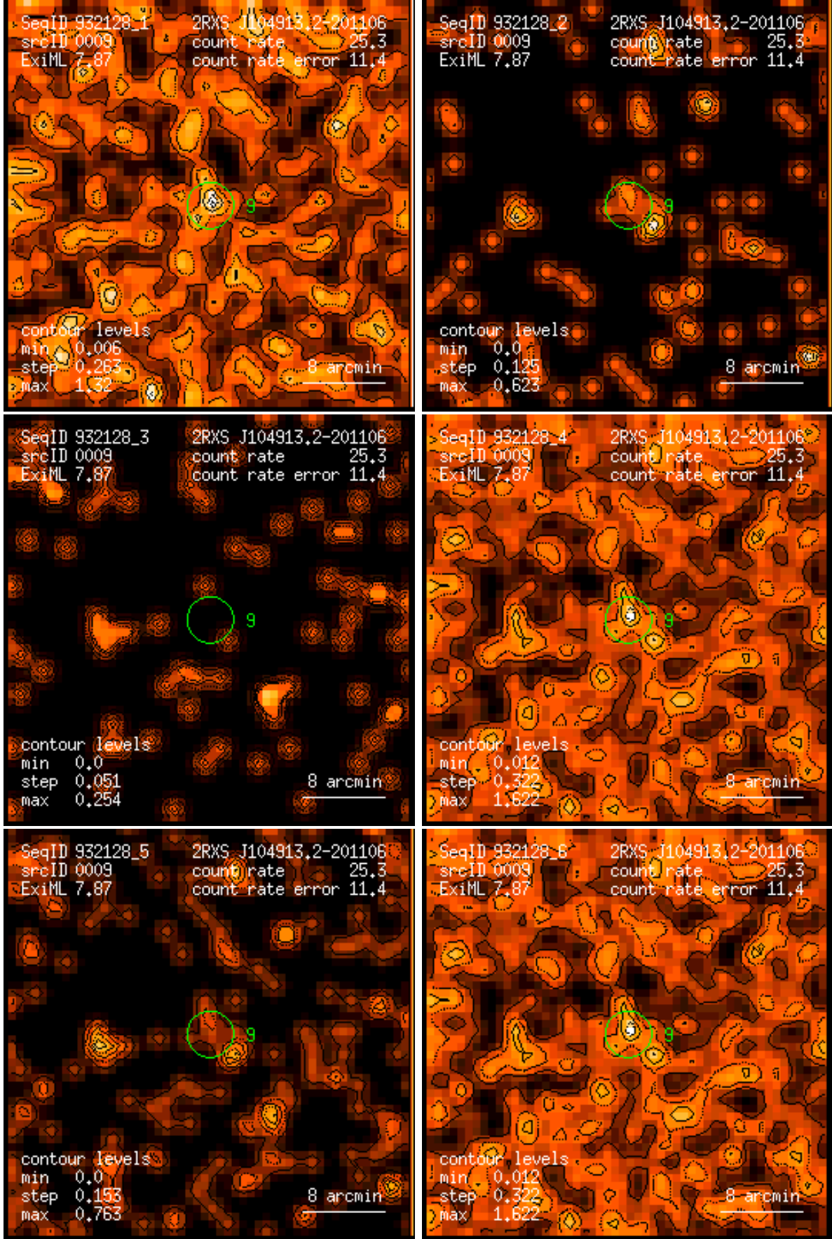
Figure 9: RASS 932128: detection 0009: band rate images, Gaussian filter: (1) PSPC channels 11 – 41, (2) 52 – 90, (3) 91 – 201, (4) 11 – 235, (5) 52 – 201, (6) 11 – 201. Broad band rates in counts/ks. Band rate contour levels in counts/ks/arcmin 2 .
