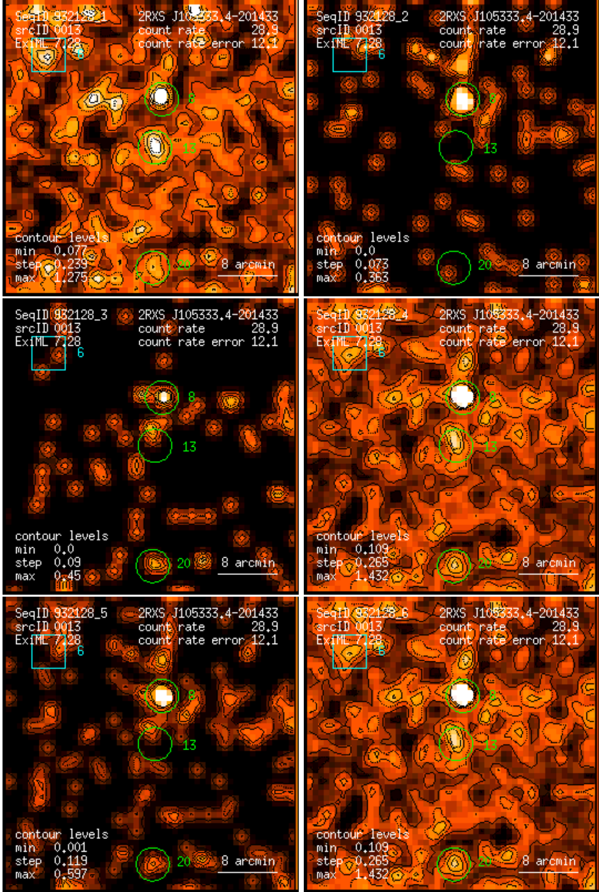
Figure 13: RASS 932128: detection 0013: band rate images, Gaussian filter: (1) PSPC channels 11 – 41, (2) 52 – 90, (3) 91 – 201, (4) 11 – 235, (5) 52 – 201, (6) 11 – 201. Broad band rates in counts/ks. Band rate contour levels in counts/ks/arcmin 2 .
