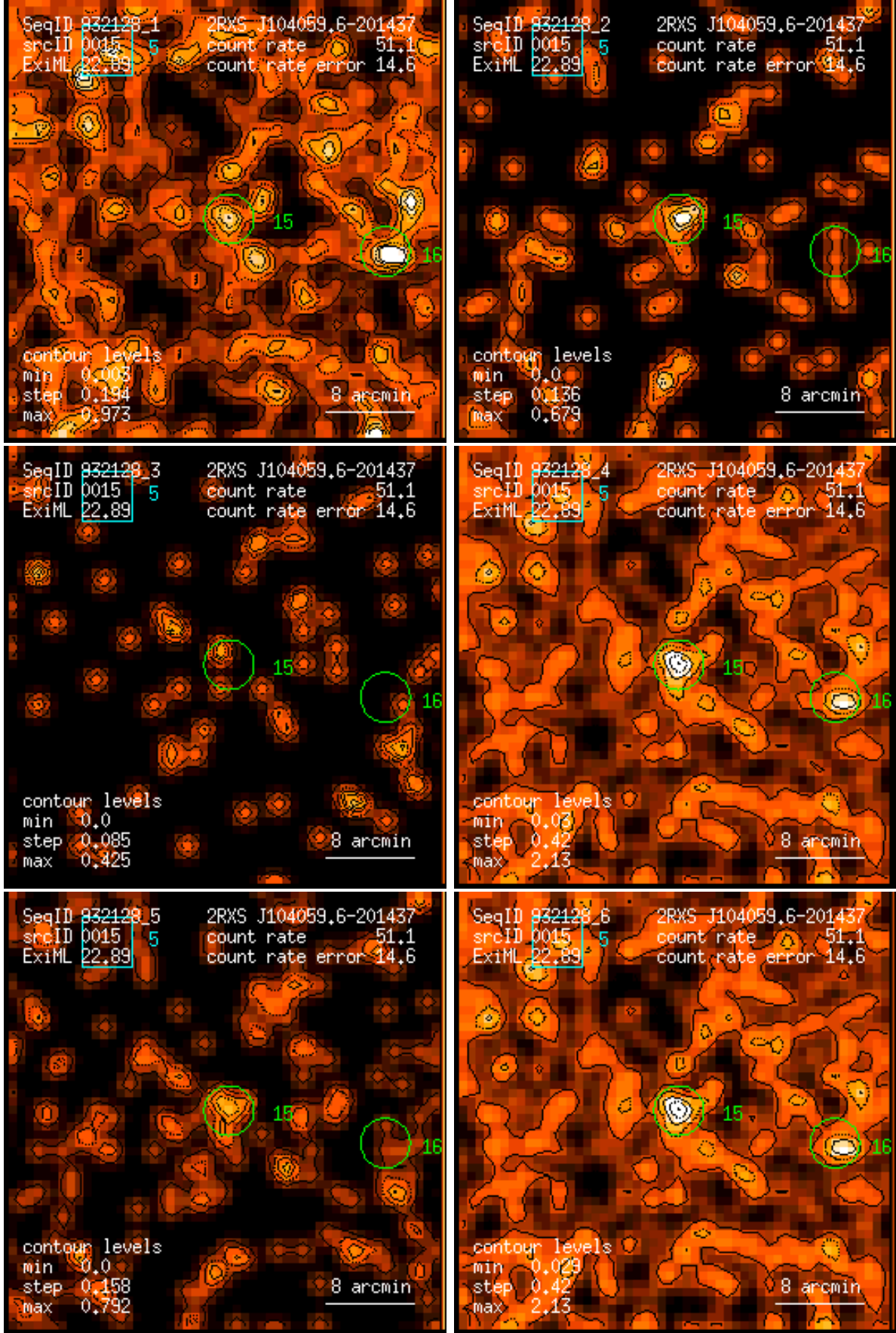
Figure 15: RASS 932128: detection 0015: band rate images, Gaussian filter: (1) PSPC channels 11 – 41, (2) 52 – 90, (3) 91 – 201, (4) 11 – 235, (5) 52 – 201, (6) 11 – 201. Broad band rates in counts/ks. Band rate contour levels in counts/ks/arcmin 2 .
