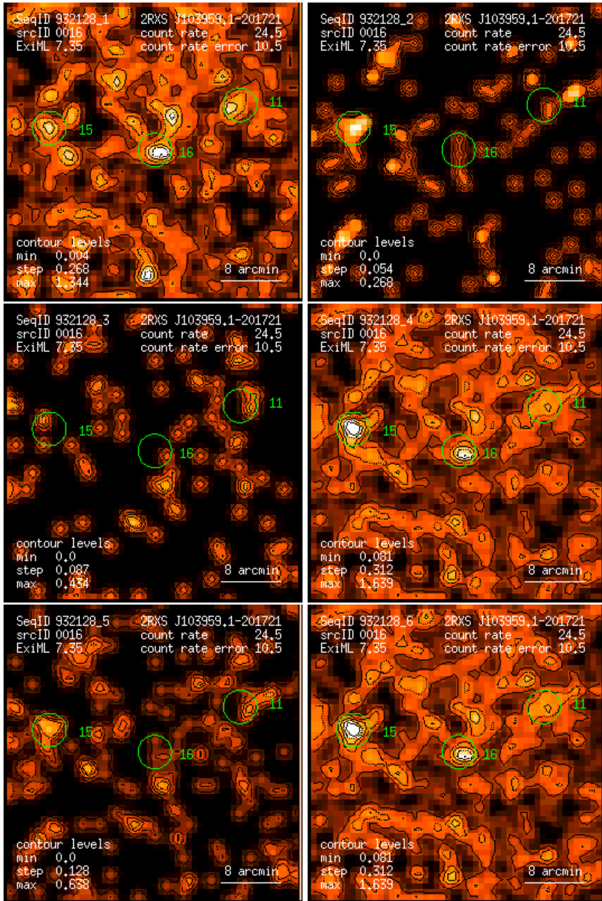
Figure 16: RASS 932128: detection 0016: band rate images, Gaussian filter: (1) PSPC channels 11 – 41, (2) 52 – 90, (3) 91 – 201, (4) 11 – 235, (5) 52 – 201, (6) 11 – 201. Broad band rates in counts/ks. Band rate contour levels in counts/ks/arcmin 2 .
