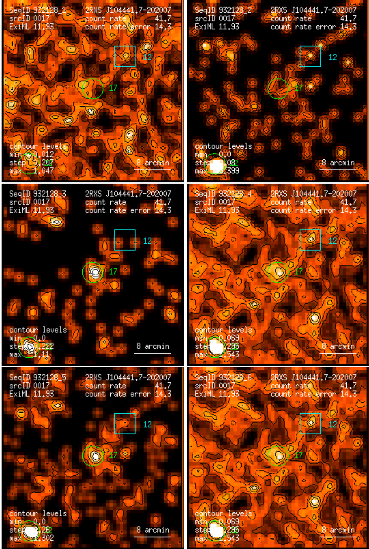
Figure 17: RASS 932128: detection 0017: band rate images, Gaussian filter: (1) PSPC channels 11 – 41, (2) 52 – 90, (3) 91 – 201, (4) 11 – 235, (5) 52 – 201, (6) 11 – 201. Broad band rates in counts/ks. Band rate contour levels in counts/ks/arcmin 2 .
