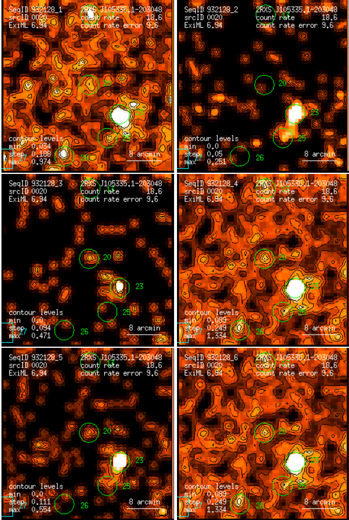
Figure 20: RASS 932128: detection 0020: band rate images, Gaussian filter: (1) PSPC channels 11 – 41, (2) 52 – 90, (3) 91 – 201, (4) 11 – 235, (5) 52 – 201, (6) 11 – 201. Broad band rates in counts/ks. Band rate contour levels in counts/ks/arcmin 2 .
