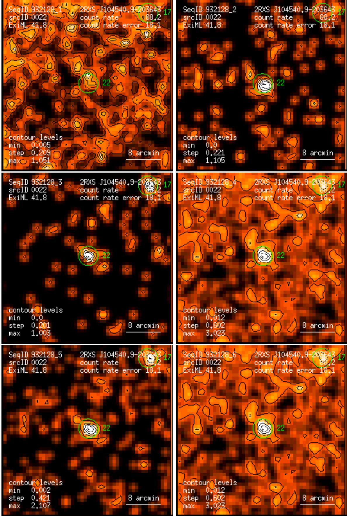
Figure 22: RASS 932128: detection 0022: band rate images, Gaussian filter: (1) PSPC channels 11 – 41, (2) 52 – 90, (3) 91 – 201, (4) 11 – 235, (5) 52 – 201, (6) 11 – 201. Broad band rates in counts/ks. Band rate contour levels in counts/ks/arcmin 2 .
