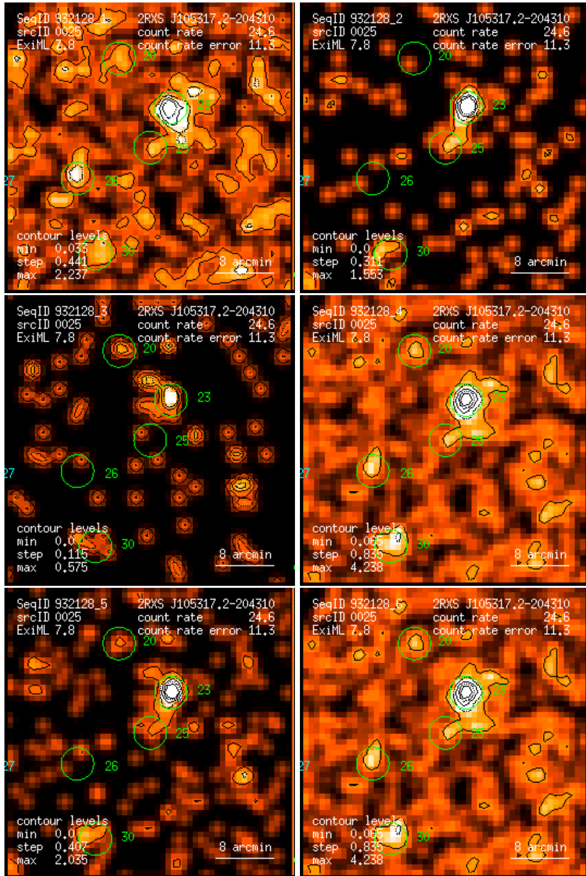
Figure 25: RASS 932128: detection 0025: band rate images, Gaussian filter: (1) PSPC channels 11 – 41, (2) 52 – 90, (3) 91 – 201, (4) 11 – 235, (5) 52 – 201, (6) 11 – 201. Broad band rates in counts/ks. Band rate contour levels in counts/ks/arcmin 2 .
