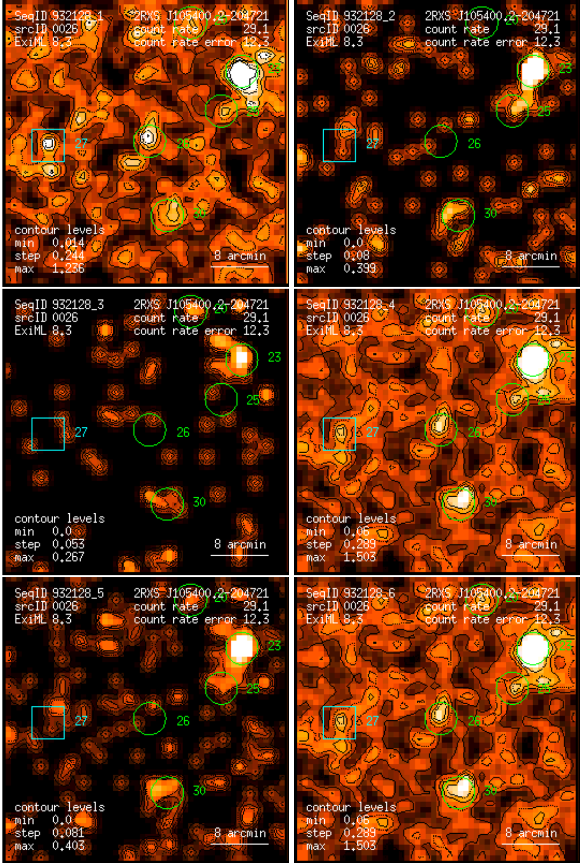
Figure 26: RASS 932128: detection 0026: band rate images, Gaussian filter: (1) PSPC channels 11 – 41, (2) 52 – 90, (3) 91 – 201, (4) 11 – 235, (5) 52 – 201, (6) 11 – 201. Broad band rates in counts/ks. Band rate contour levels in counts/ks/arcmin 2 .
