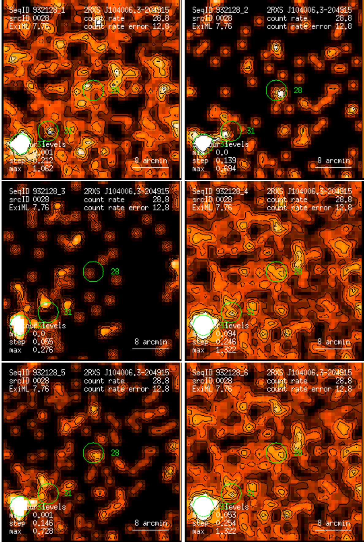
Figure 28: RASS 932128: detection 0028: band rate images, Gaussian filter: (1) PSPC channels 11 – 41, (2) 52 – 90, (3) 91 – 201, (4) 11 – 235, (5) 52 – 201, (6) 11 – 201. Broad band rates in counts/ks. Band rate contour levels in counts/ks/arcmin 2 .
