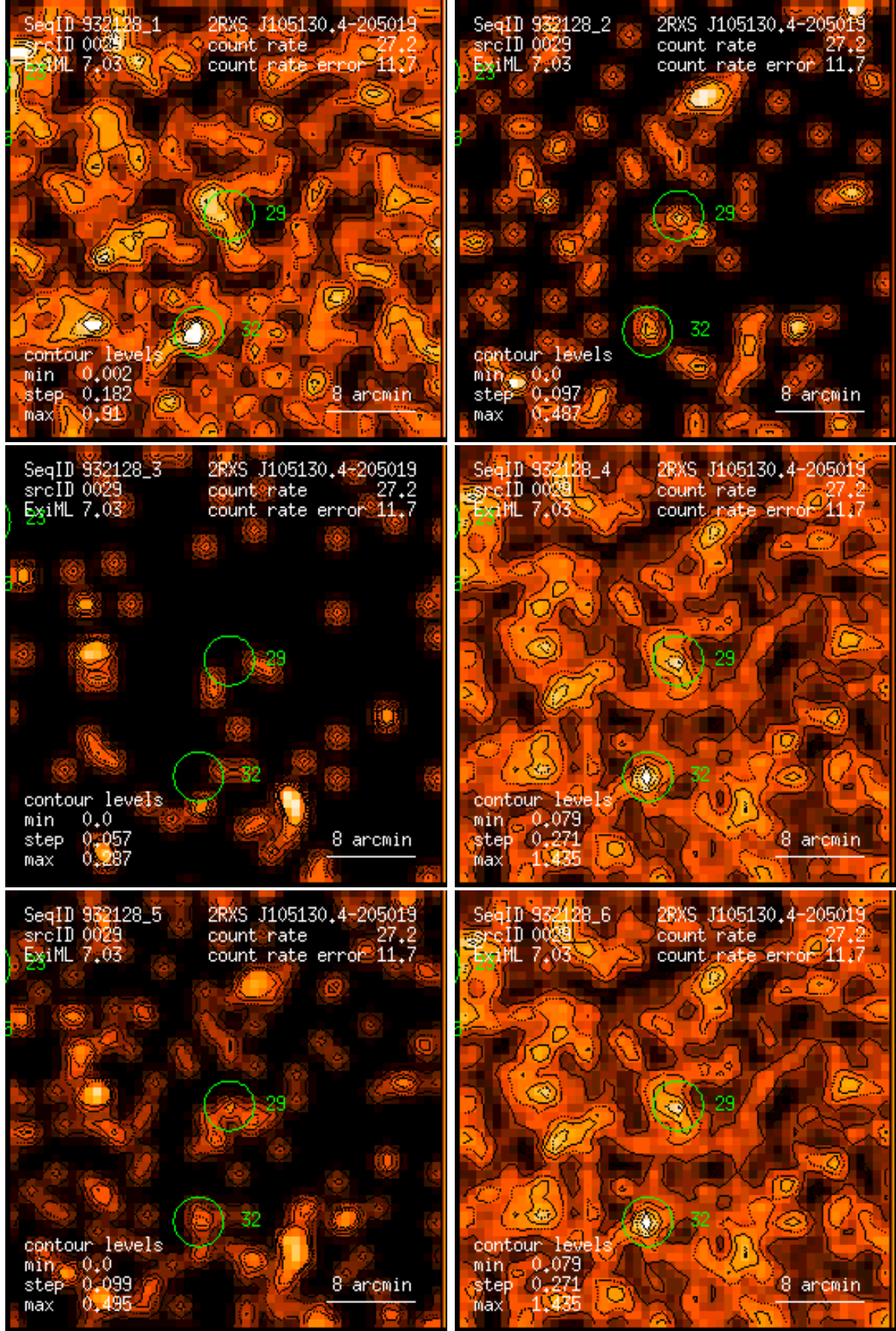
Figure 29: RASS 932128: detection 0029: band rate images, Gaussian filter: (1) PSPC channels 11 – 41, (2) 52 – 90, (3) 91 – 201, (4) 11 – 235, (5) 52 – 201, (6) 11 – 201. Broad band rates in counts/ks. Band rate contour levels in counts/ks/arcmin 2 .
