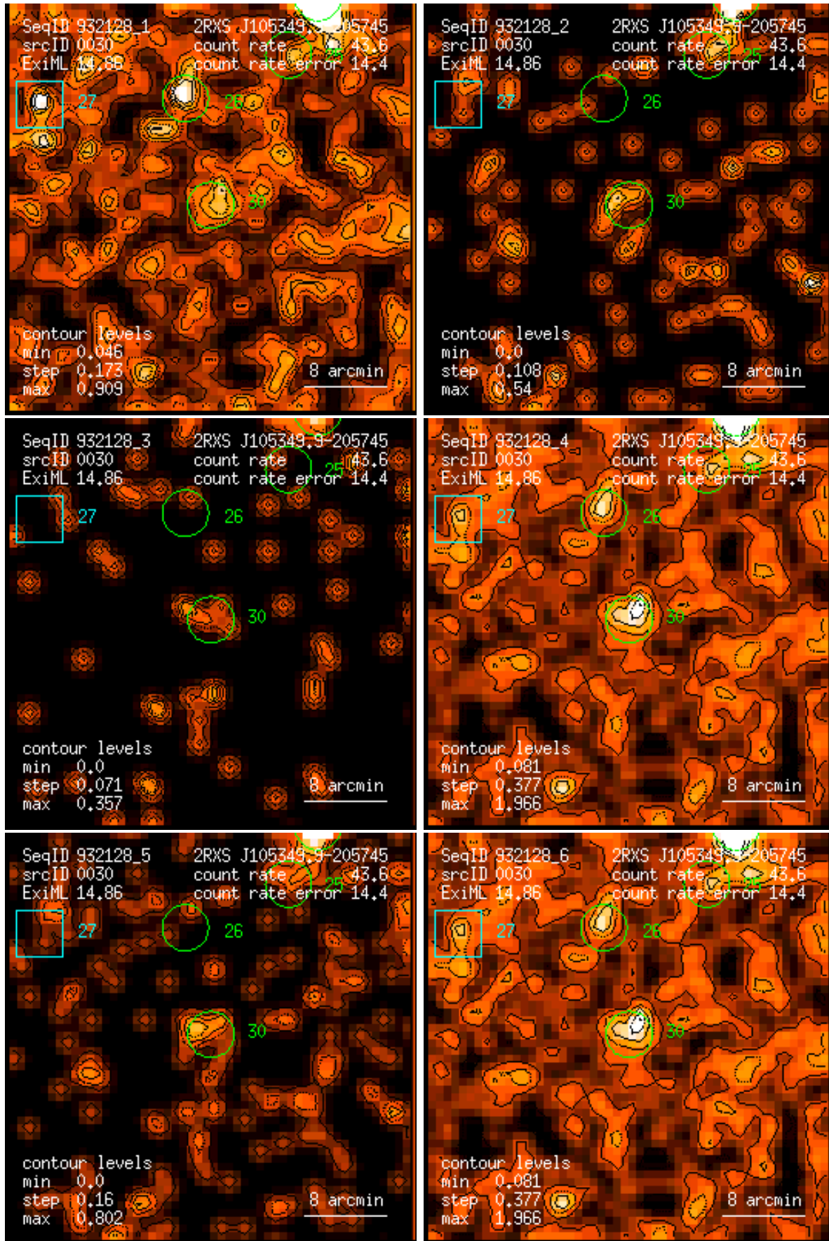
Figure 30: RASS 932128: detection 0030: band rate images, Gaussian filter: (1) PSPC channels 11 – 41, (2) 52 – 90, (3) 91 – 201, (4) 11 – 235, (5) 52 – 201, (6) 11 – 201. Broad band rates in counts/ks. Band rate contour levels in counts/ks/arcmin 2 .
