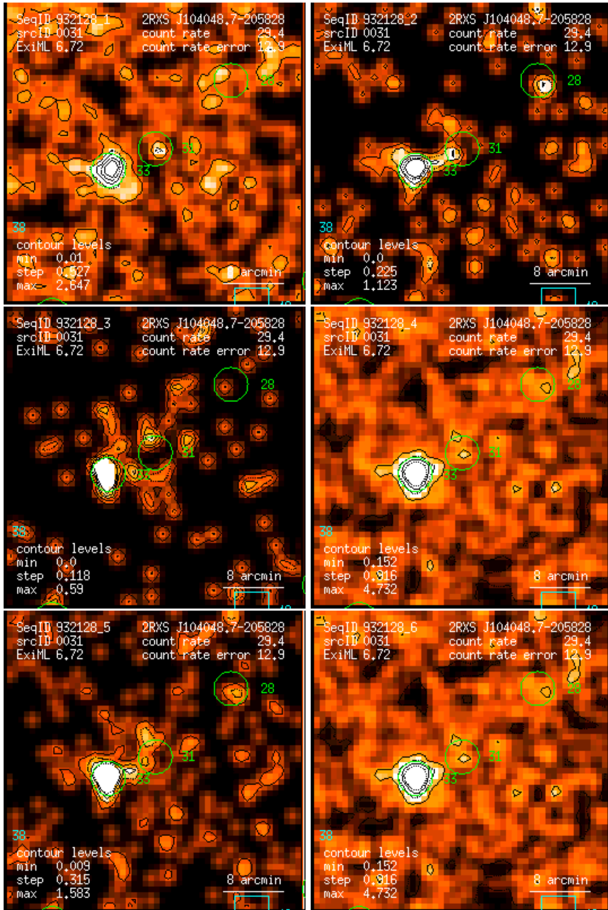
Figure 31: RASS 932128: detection 0031: band rate images, Gaussian filter: (1) PSPC channels 11 – 41, (2) 52 – 90, (3) 91 – 201, (4) 11 – 235, (5) 52 – 201, (6) 11 – 201. Broad band rates in counts/ks. Band rate contour levels in counts/ks/arcmin 2 .
