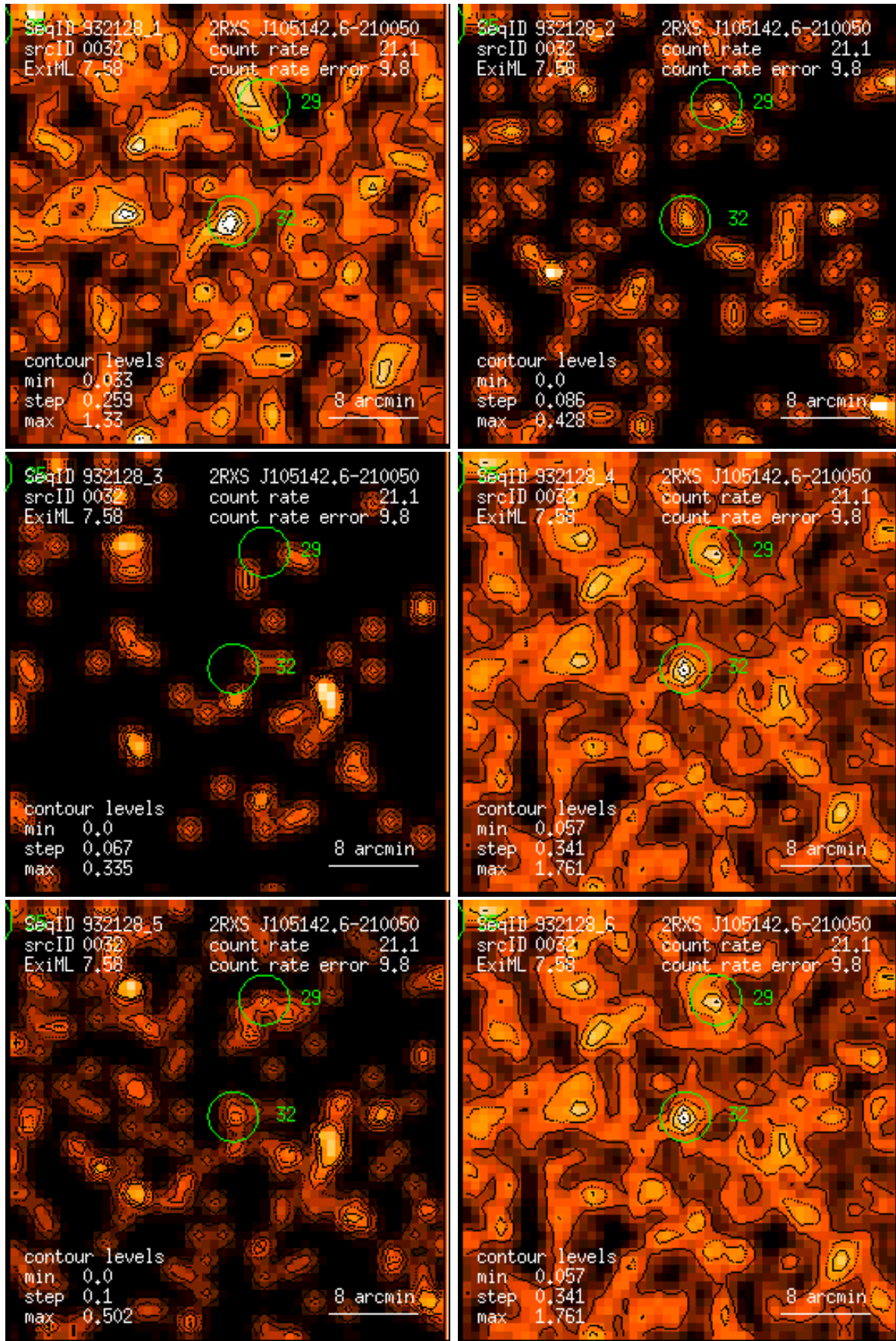
Figure 32: RASS 932128: detection 0032: band rate images, Gaussian filter: (1) PSPC channels 11 – 41, (2) 52 – 90, (3) 91 – 201, (4) 11 – 235, (5) 52 – 201, (6) 11 – 201. Broad band rates in counts/ks. Band rate contour levels in counts/ks/arcmin 2 .
