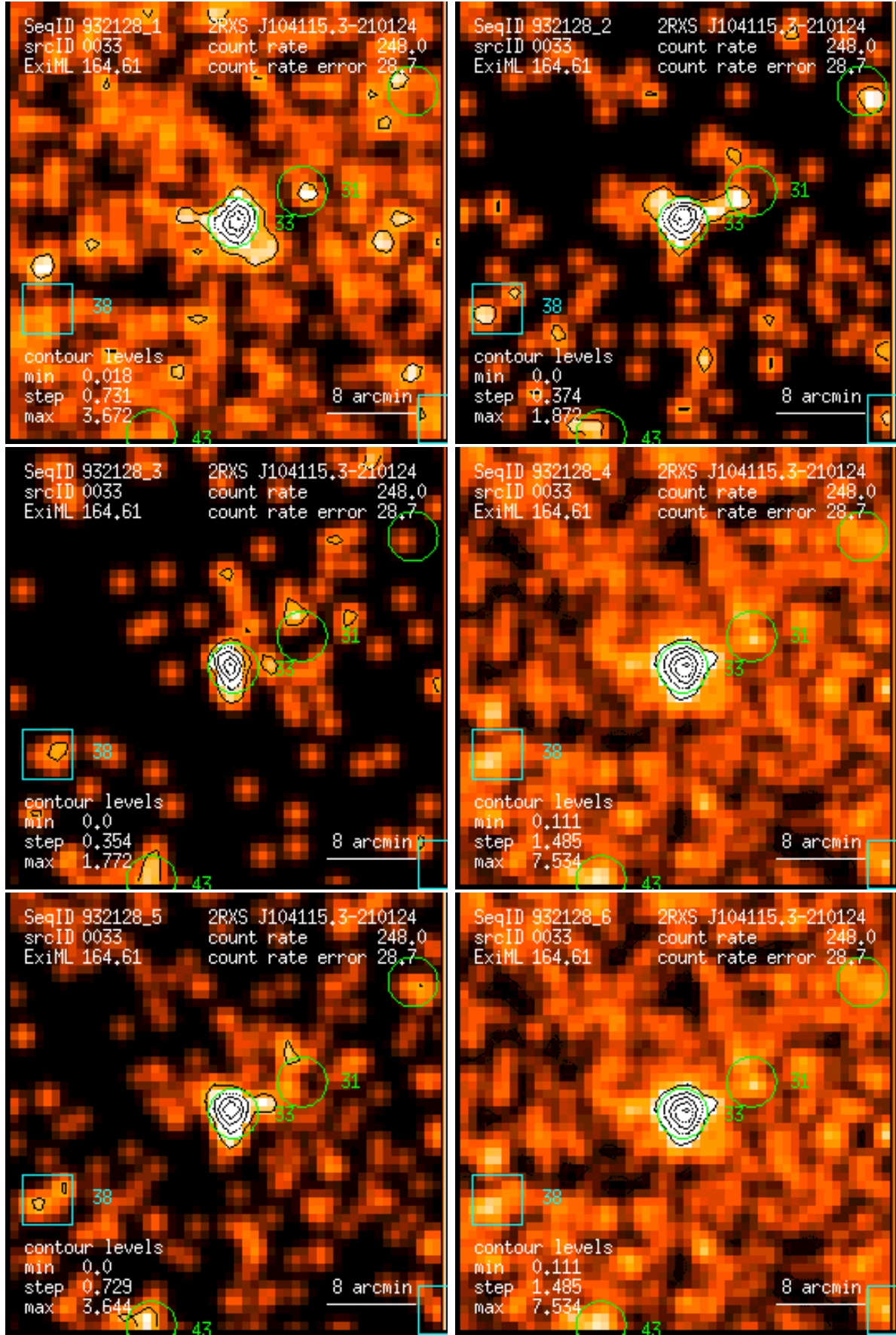
Figure 33: RASS 932128: detection 0033: band rate images, Gaussian filter: (1) PSPC channels 11 – 41, (2) 52 – 90, (3) 91 – 201, (4) 11 – 235, (5) 52 – 201, (6) 11 – 201. Broad band rates in counts/ks. Band rate contour levels in counts/ks/arcmin 2 .
