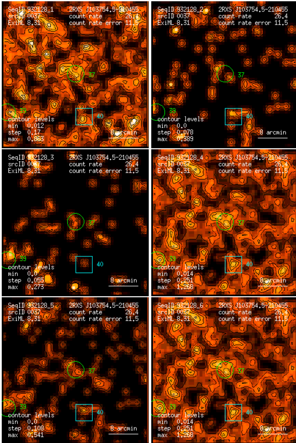
Figure 37: RASS 932128: detection 0037: band rate images, Gaussian filter: (1) PSPC channels 11 – 41, (2) 52 – 90, (3) 91 – 201, (4) 11 – 235, (5) 52 – 201, (6) 11 – 201. Broad band rates in counts/ks. Band rate contour levels in counts/ks/arcmin 2 .
