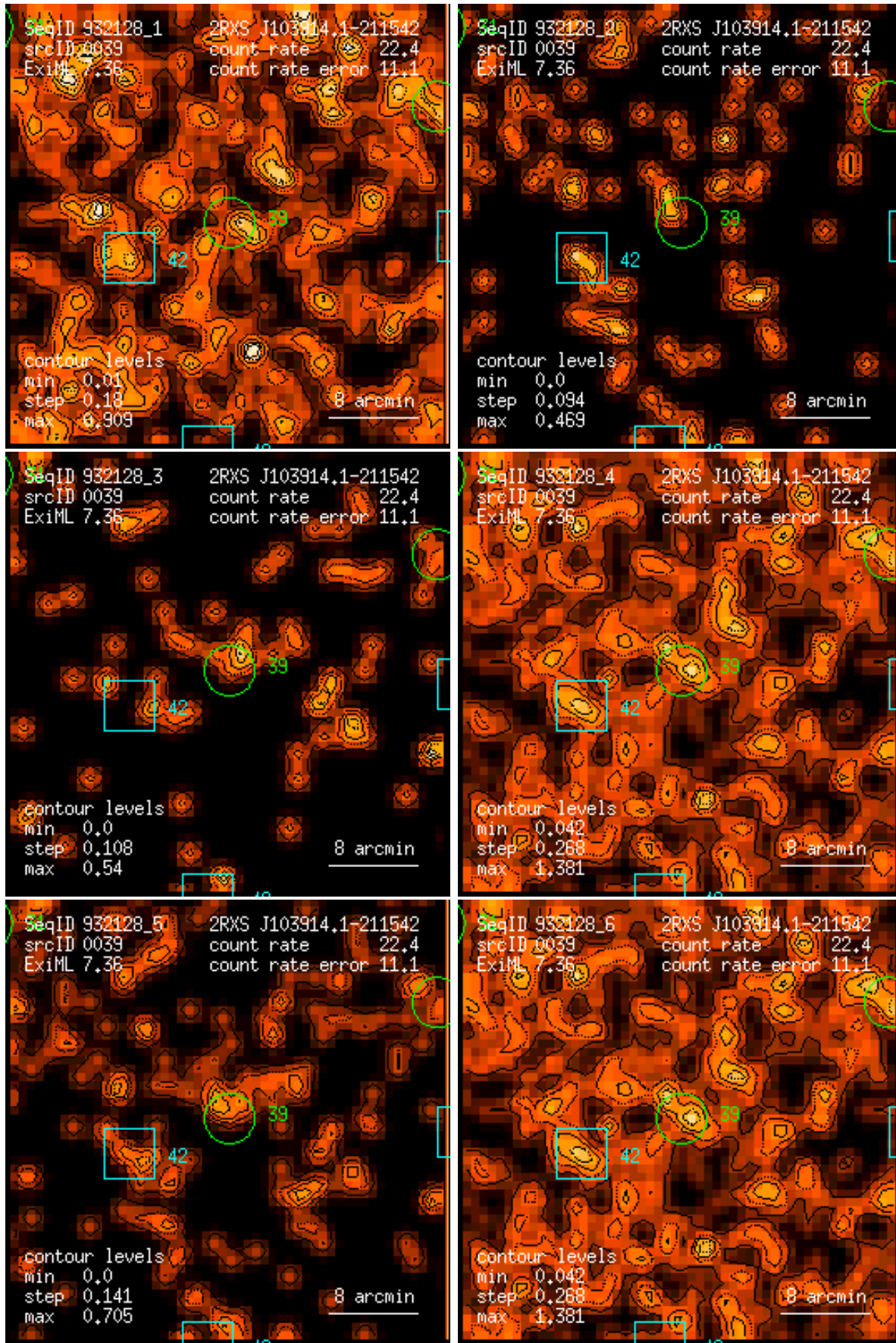
Figure 39: RASS 932128: detection 0039: band rate images, Gaussian filter: (1) PSPC channels 11 – 41, (2) 52 – 90, (3) 91 – 201, (4) 11 – 235, (5) 52 – 201, (6) 11 – 201. Broad band rates in counts/ks. Band rate contour levels in counts/ks/arcmin 2 .
