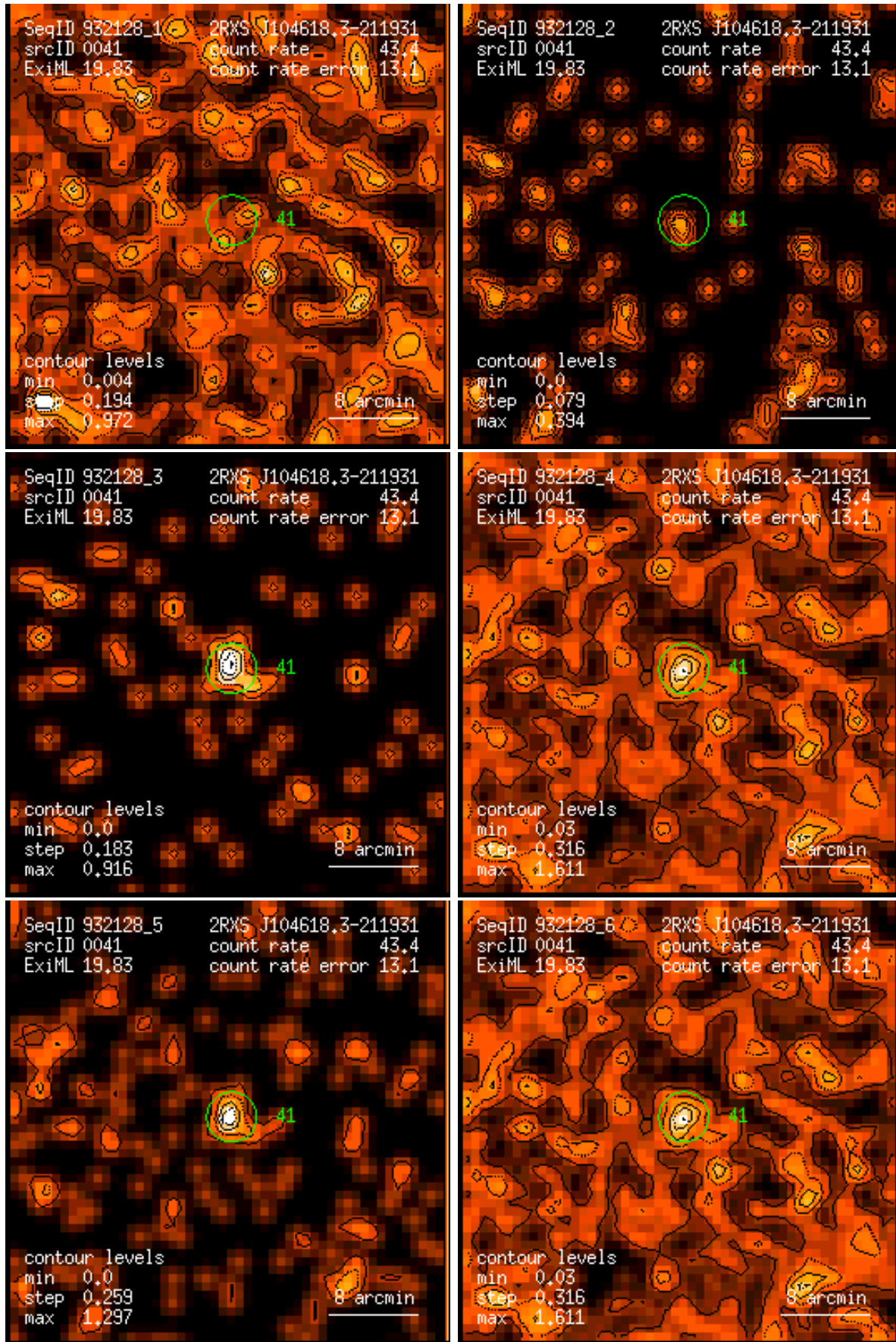
Figure 41: RASS 932128: detection 0041: band rate images, Gaussian filter: (1) PSPC channels 11 – 41, (2) 52 – 90, (3) 91 – 201, (4) 11 – 235, (5) 52 – 201, (6) 11 – 201. Broad band rates in counts/ks. Band rate contour levels in counts/ks/arcmin 2 .
