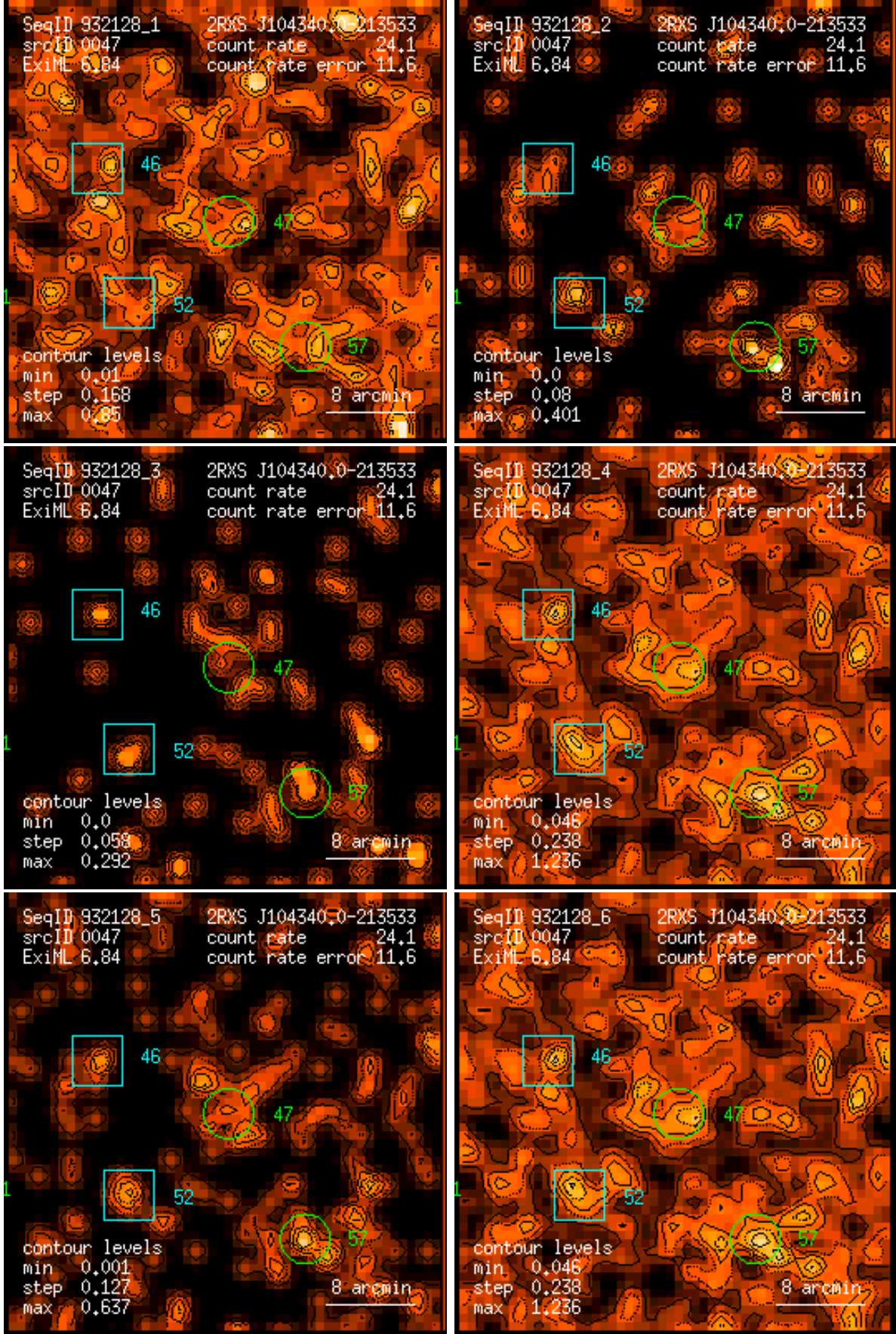
Figure 47: RASS 932128: detection 0047: band rate images, Gaussian filter: (1) PSPC channels 11 – 41, (2) 52 – 90, (3) 91 – 201, (4) 11 – 235, (5) 52 – 201, (6) 11 – 201. Broad band rates in counts/ks. Band rate contour levels in counts/ks/arcmin 2 .
