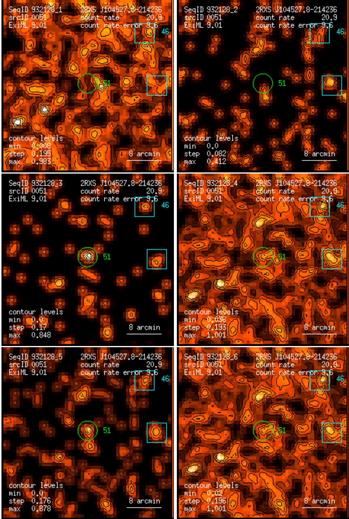
Figure 51: RASS 932128: detection 0051: band rate images, Gaussian filter: (1) PSPC channels 11 – 41, (2) 52 – 90, (3) 91 – 201, (4) 11 – 235, (5) 52 – 201, (6) 11 – 201. Broad band rates in counts/ks. Band rate contour levels in counts/ks/arcmin 2 .
