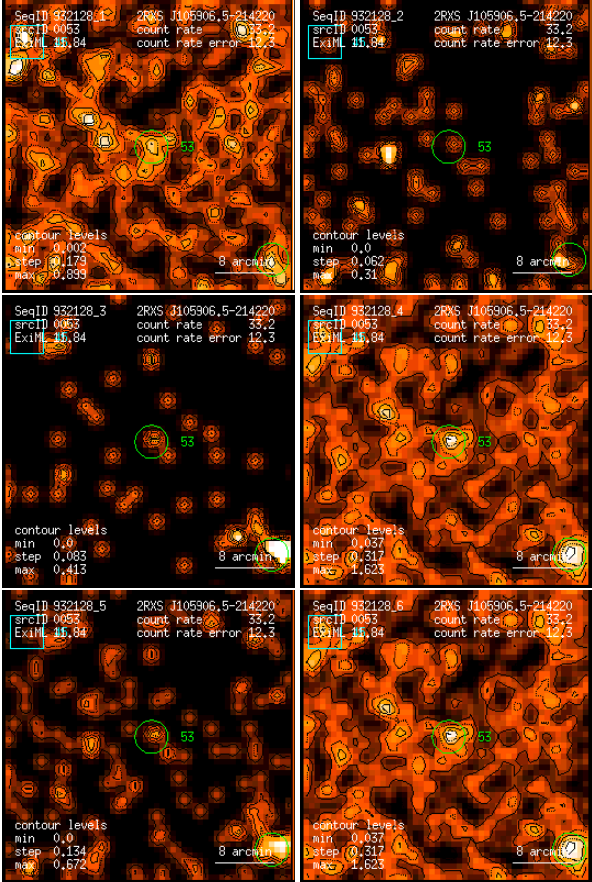
Figure 53: RASS 932128: detection 0053: band rate images, Gaussian filter: (1) PSPC channels 11 – 41, (2) 52 – 90, (3) 91 – 201, (4) 11 – 235, (5) 52 – 201, (6) 11 – 201. Broad band rates in counts/ks. Band rate contour levels in counts/ks/arcmin 2 .
