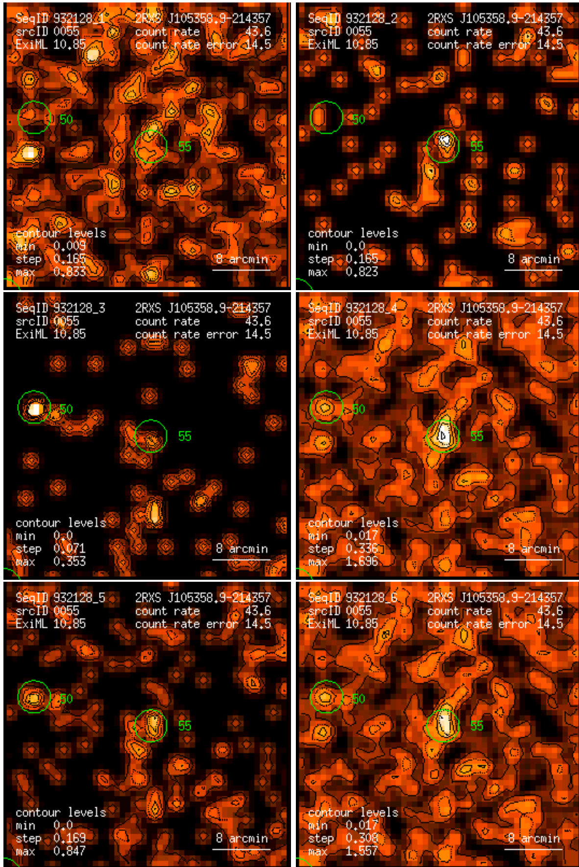
Figure 55: RASS 932128: detection 0055: band rate images, Gaussian filter: (1) PSPC channels 11 – 41, (2) 52 – 90, (3) 91 – 201, (4) 11 – 235, (5) 52 – 201, (6) 11 – 201. Broad band rates in counts/ks. Band rate contour levels in counts/ks/arcmin 2 .
