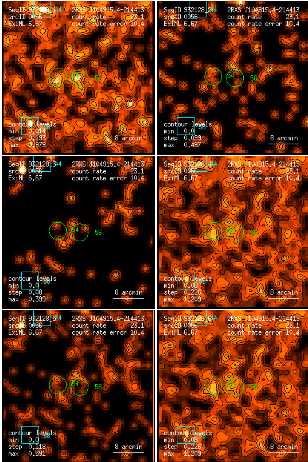
Figure 56: RASS 932128: detection 0056: band rate images, Gaussian filter: (1) PSPC channels 11 – 41, (2) 52 – 90, (3) 91 – 201, (4) 11 – 235, (5) 52 – 201, (6) 11 – 201. Broad band rates in counts/ks. Band rate contour levels in counts/ks/arcmin 2 .
