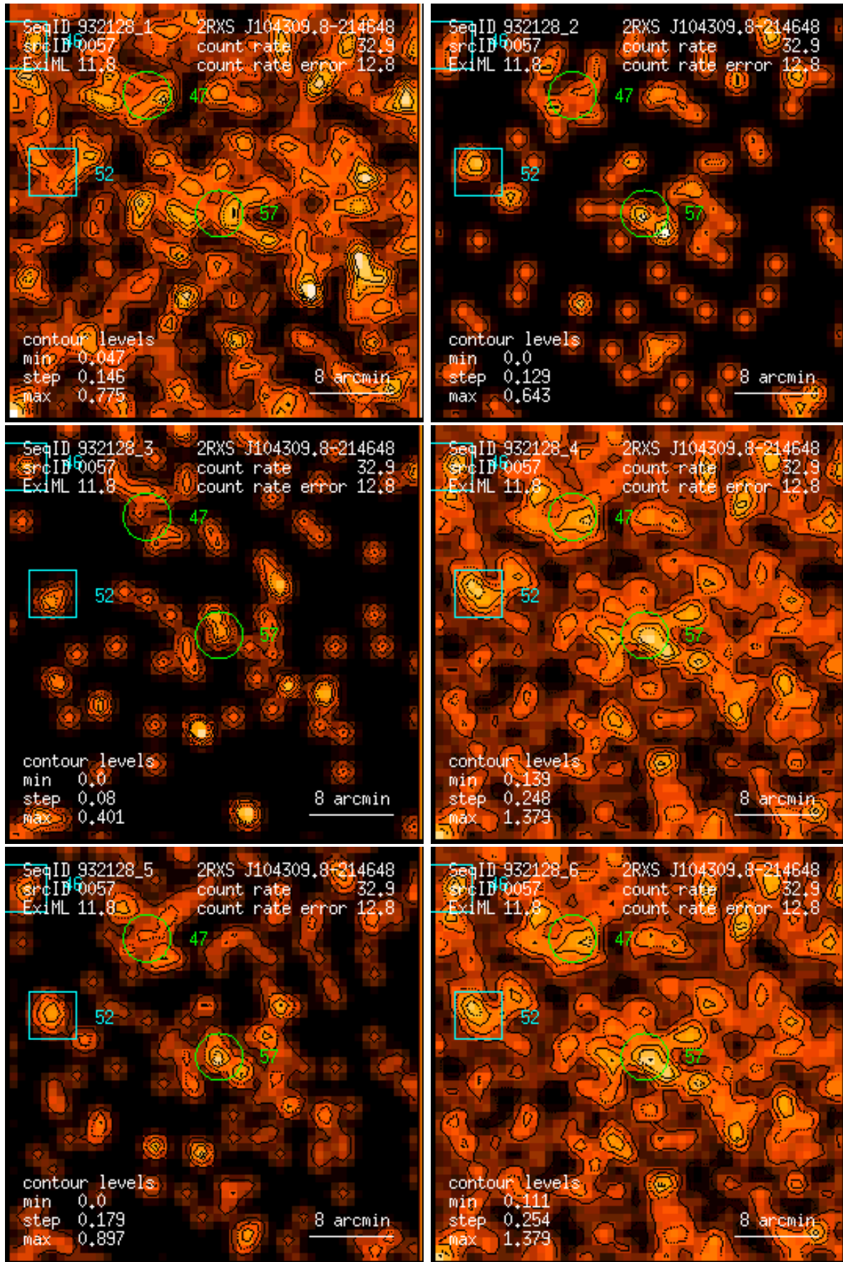
Figure 57: RASS 932128: detection 0057: band rate images, Gaussian filter: (1) PSPC channels 11 – 41, (2) 52 – 90, (3) 91 – 201, (4) 11 – 235, (5) 52 – 201, (6) 11 – 201. Broad band rates in counts/ks. Band rate contour levels in counts/ks/arcmin 2 .
