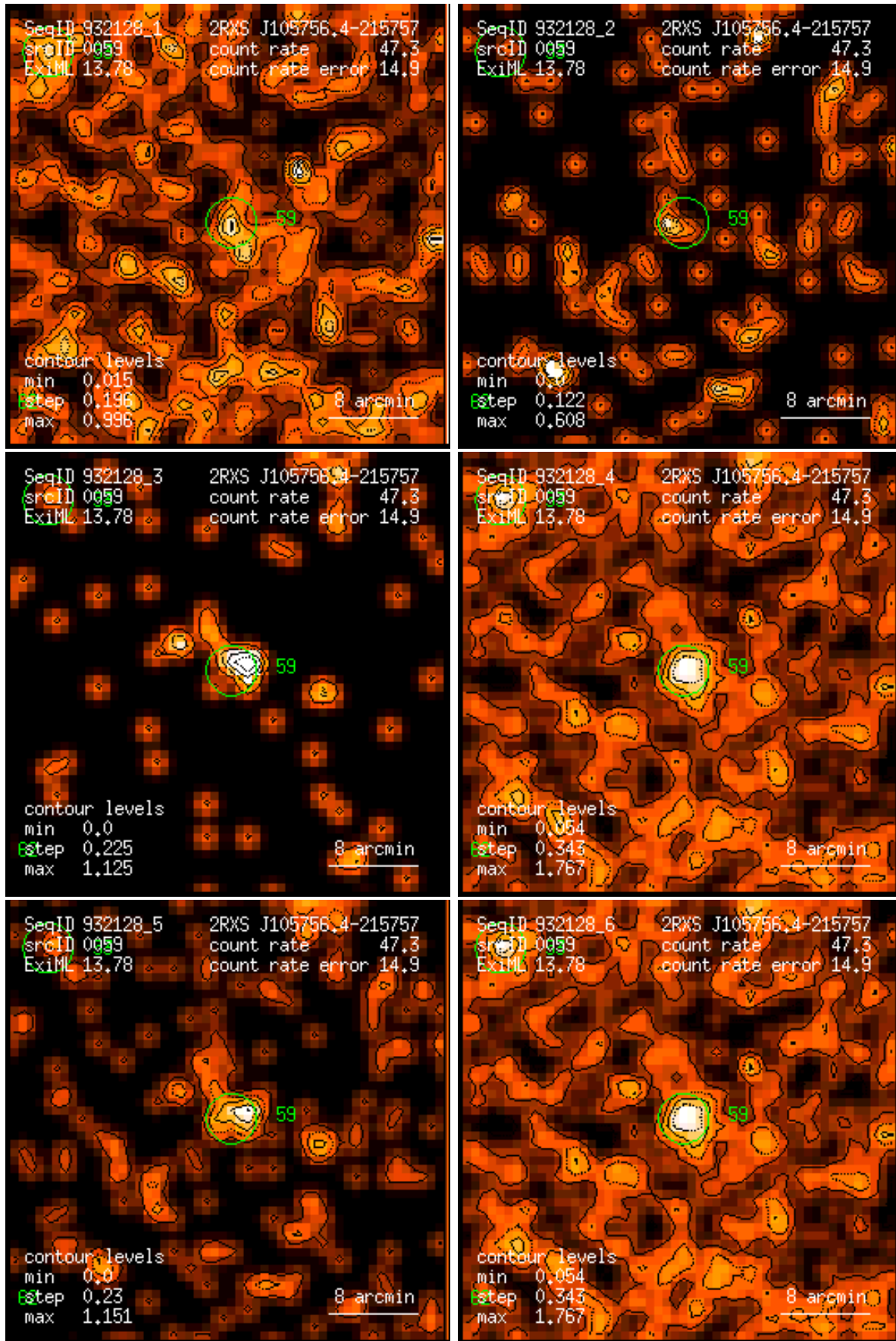
Figure 59: RASS 932128: detection 0059: band rate images, Gaussian filter: (1) PSPC channels 11 – 41, (2) 52 – 90, (3) 91 – 201, (4) 11 – 235, (5) 52 – 201, (6) 11 – 201. Broad band rates in counts/ks. Band rate contour levels in counts/ks/arcmin 2 .
