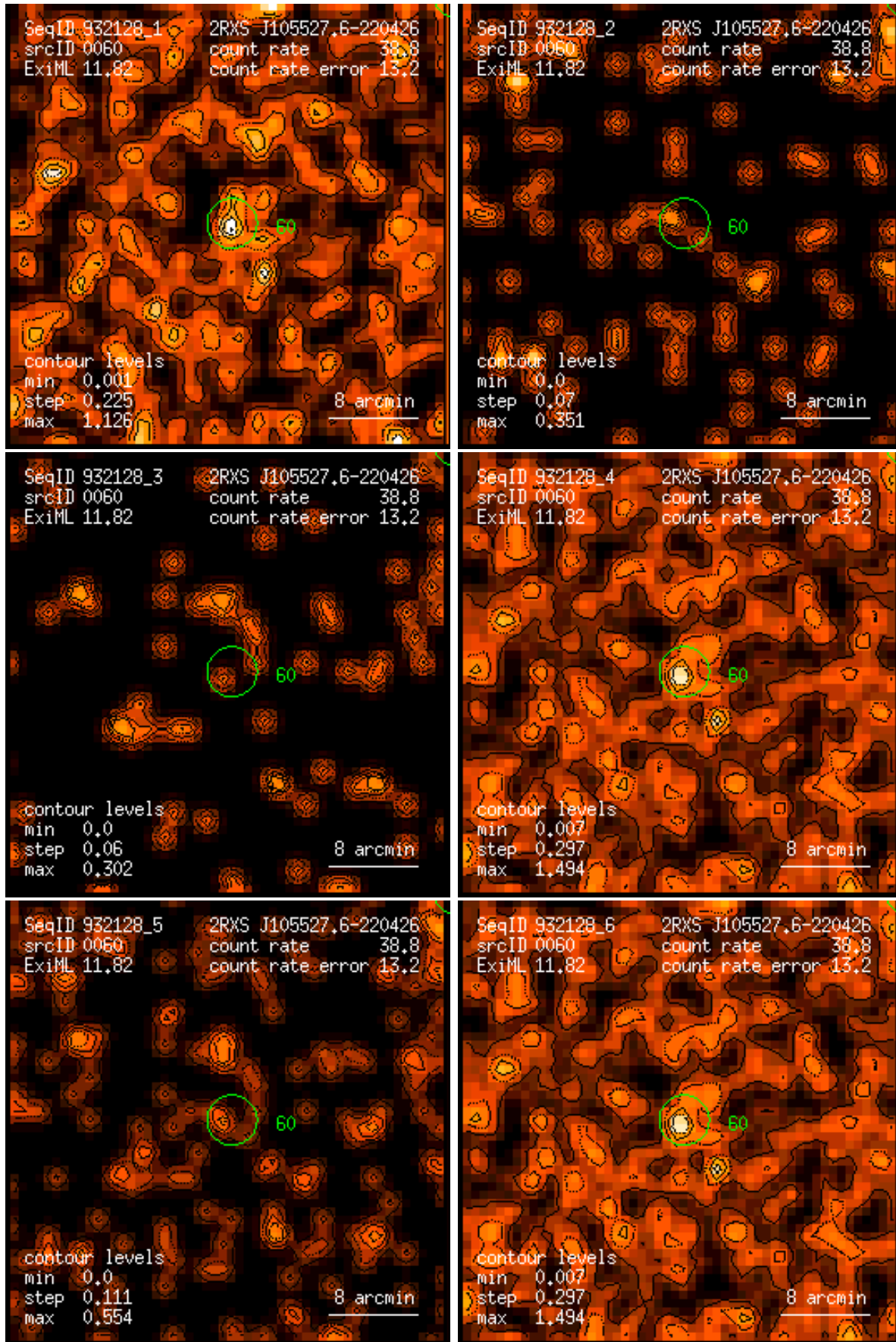
Figure 60: RASS 932128: detection 0060: band rate images, Gaussian filter: (1) PSPC channels 11 – 41, (2) 52 – 90, (3) 91 – 201, (4) 11 – 235, (5) 52 – 201, (6) 11 – 201. Broad band rates in counts/ks. Band rate contour levels in counts/ks/arcmin 2 .
