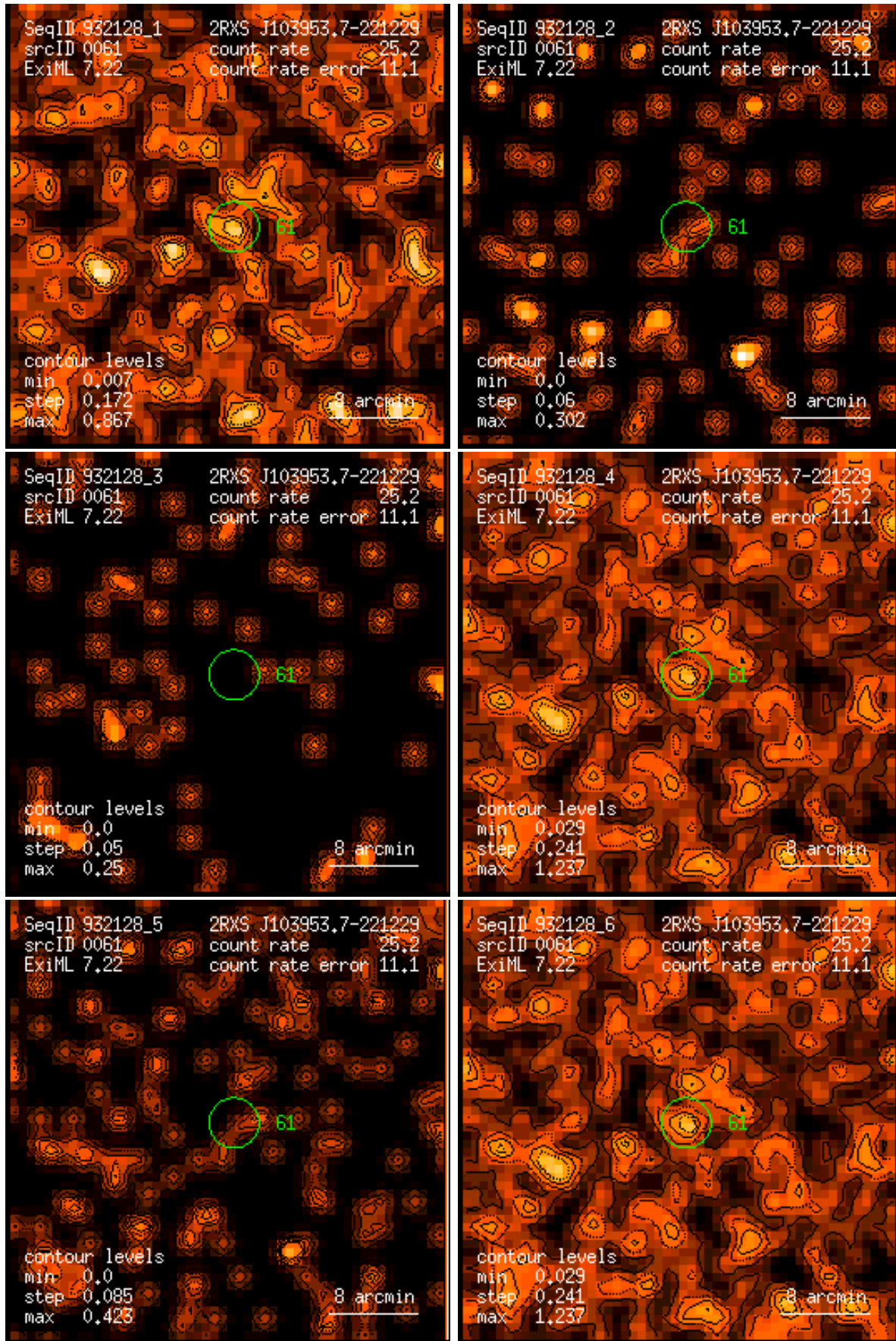
Figure 61: RASS 932128: detection 0061: band rate images, Gaussian filter: (1) PSPC channels 11 – 41, (2) 52 – 90, (3) 91 – 201, (4) 11 – 235, (5) 52 – 201, (6) 11 – 201. Broad band rates in counts/ks. Band rate contour levels in counts/ks/arcmin 2 .
