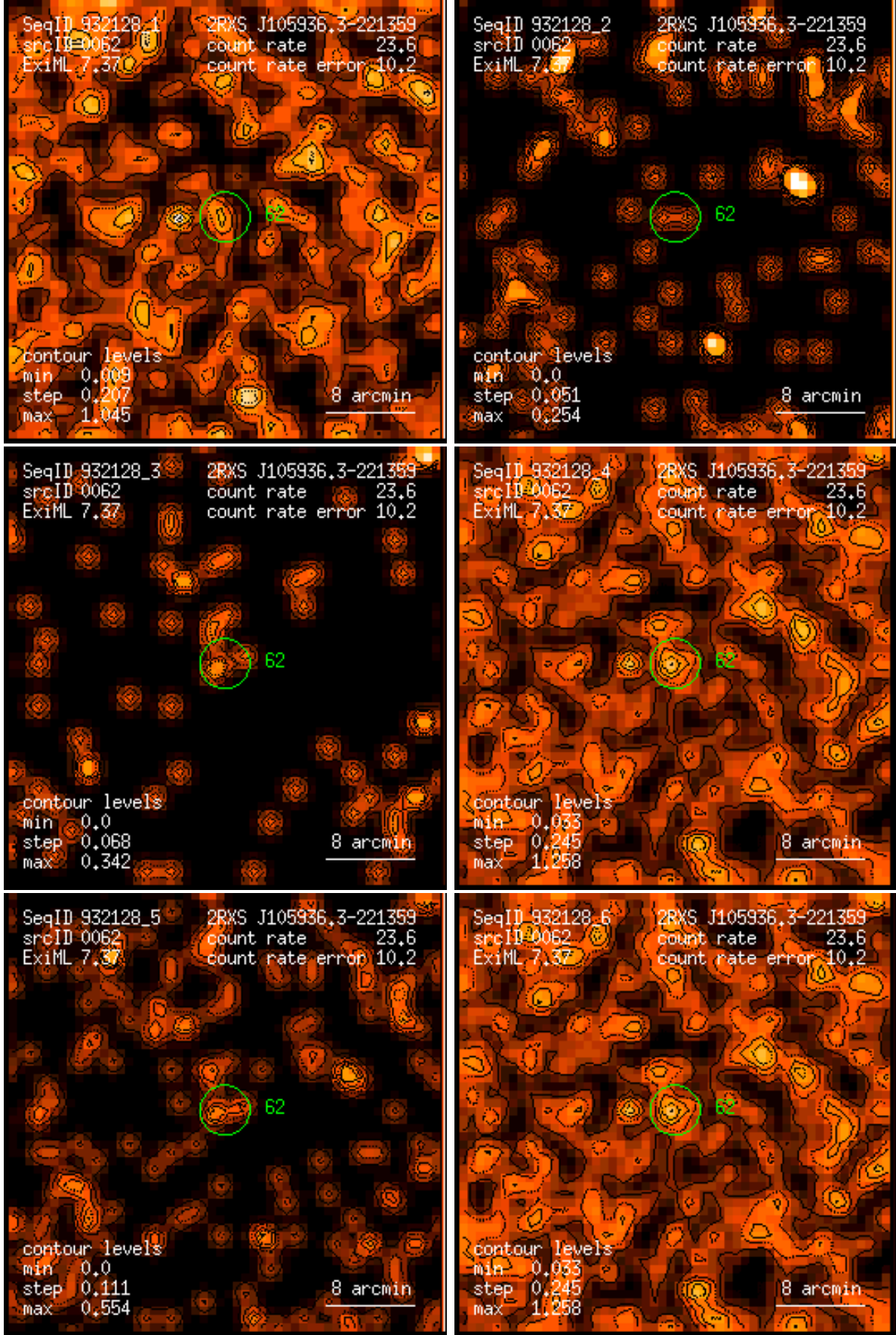
Figure 62: RASS 932128: detection 0062: band rate images, Gaussian filter: (1) PSPC channels 11 – 41, (2) 52 – 90, (3) 91 – 201, (4) 11 – 235, (5) 52 – 201, (6) 11 – 201. Broad band rates in counts/ks. Band rate contour levels in counts/ks/arcmin 2 .
