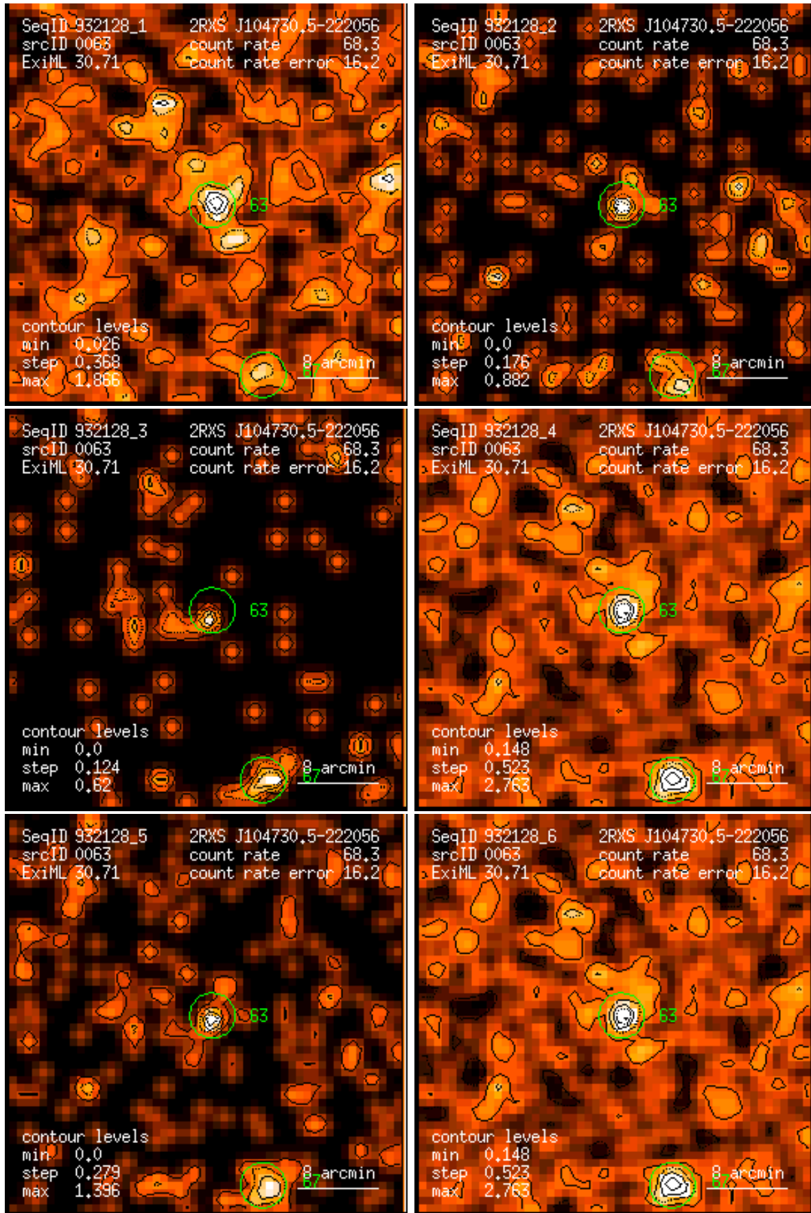
Figure 63: RASS 932128: detection 0063: band rate images, Gaussian filter: (1) PSPC channels 11 – 41, (2) 52 – 90, (3) 91 – 201, (4) 11 – 235, (5) 52 – 201, (6) 11 – 201. Broad band rates in counts/ks. Band rate contour levels in counts/ks/arcmin 2 .
