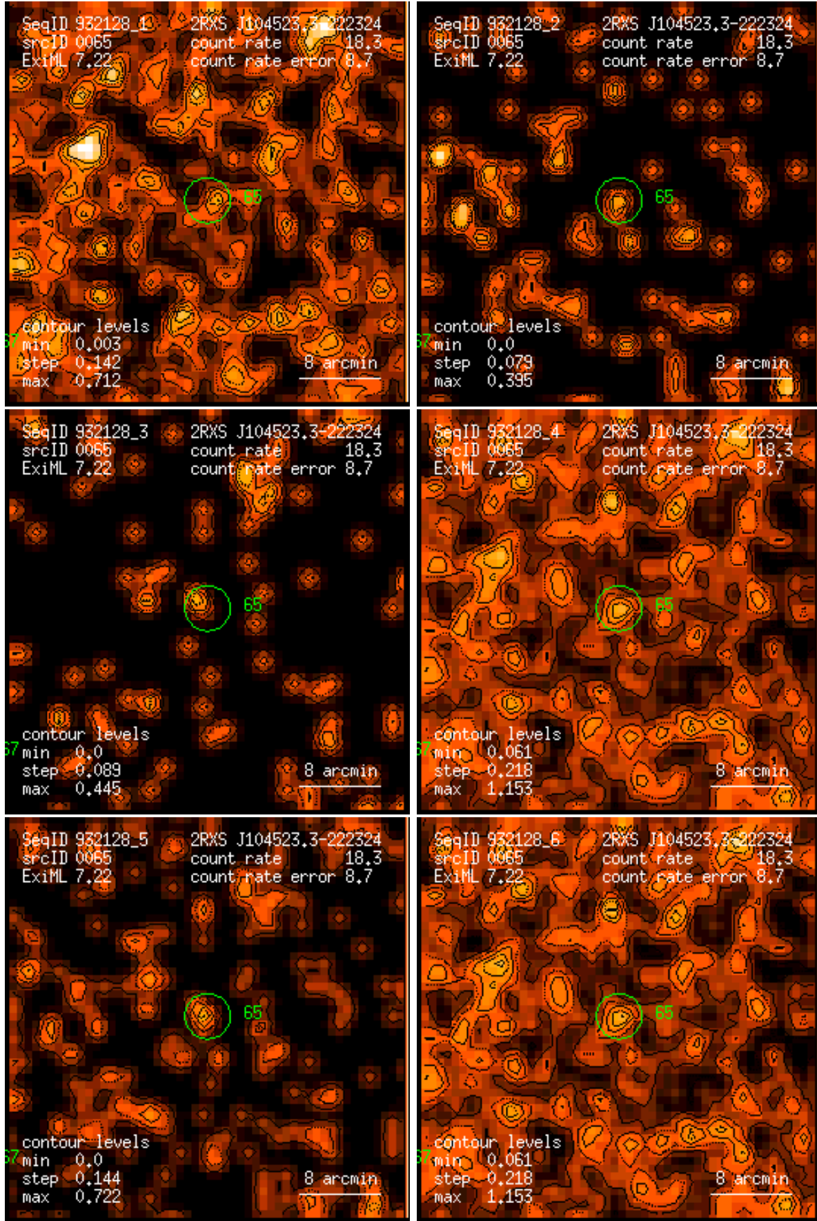
Figure 65: RASS 932128: detection 0065: band rate images, Gaussian filter: (1) PSPC channels 11 – 41, (2) 52 – 90, (3) 91 – 201, (4) 11 – 235, (5) 52 – 201, (6) 11 – 201. Broad band rates in counts/ks. Band rate contour levels in counts/ks/arcmin 2 .
