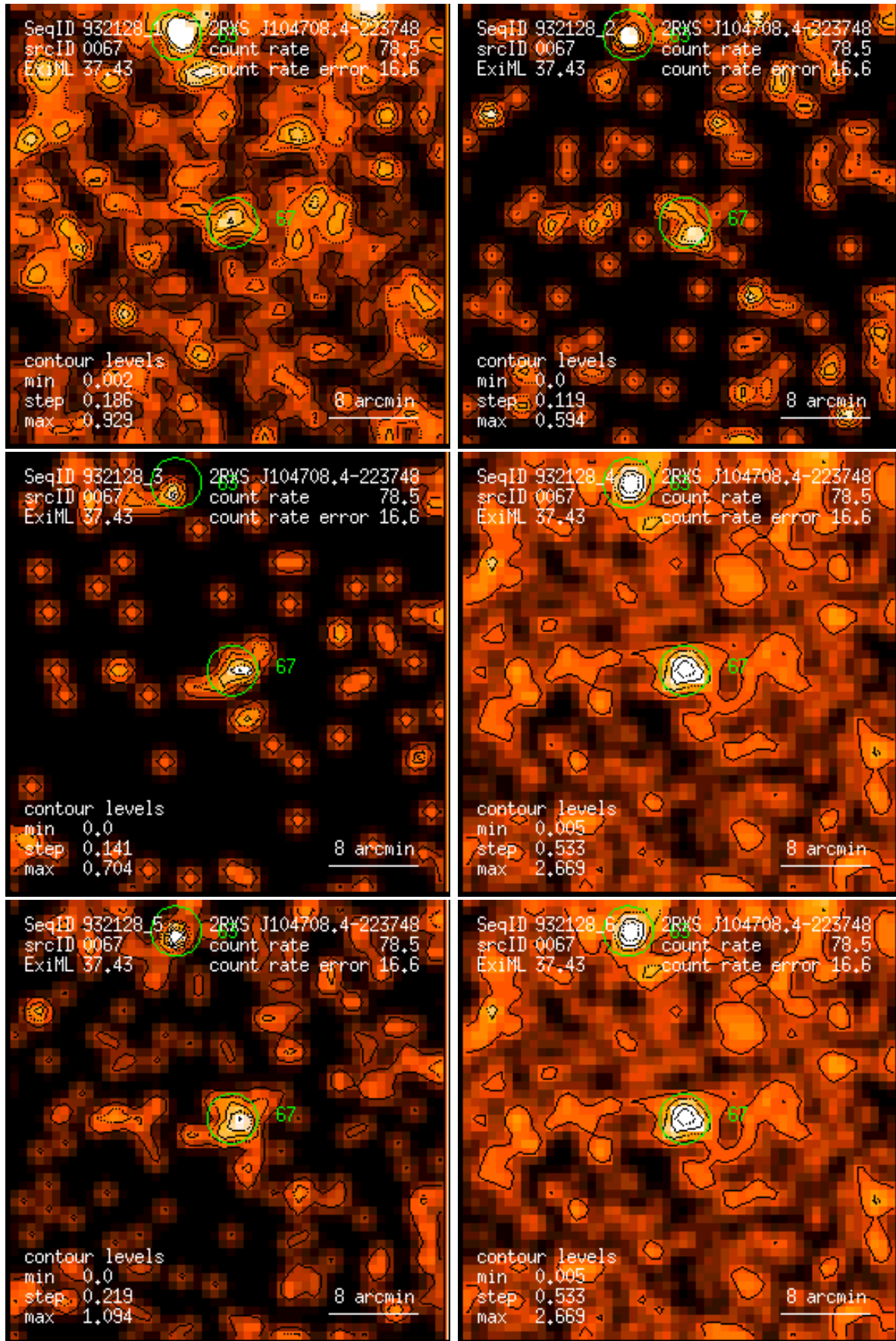
Figure 67: RASS 932128: detection 0067: band rate images, Gaussian filter: (1) PSPC channels 11 – 41, (2) 52 – 90, (3) 91 – 201, (4) 11 – 235, (5) 52 – 201, (6) 11 – 201. Broad band rates in counts/ks. Band rate contour levels in counts/ks/arcmin 2 .
