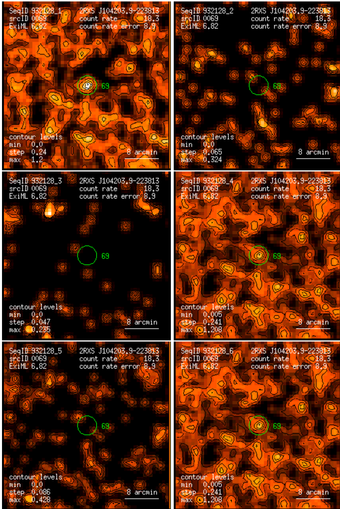
Figure 69: RASS 932128: detection 0069: band rate images, Gaussian filter: (1) PSPC channels 11 – 41, (2) 52 – 90, (3) 91 – 201, (4) 11 – 235, (5) 52 – 201, (6) 11 – 201. Broad band rates in counts/ks. Band rate contour levels in counts/ks/arcmin 2 .
