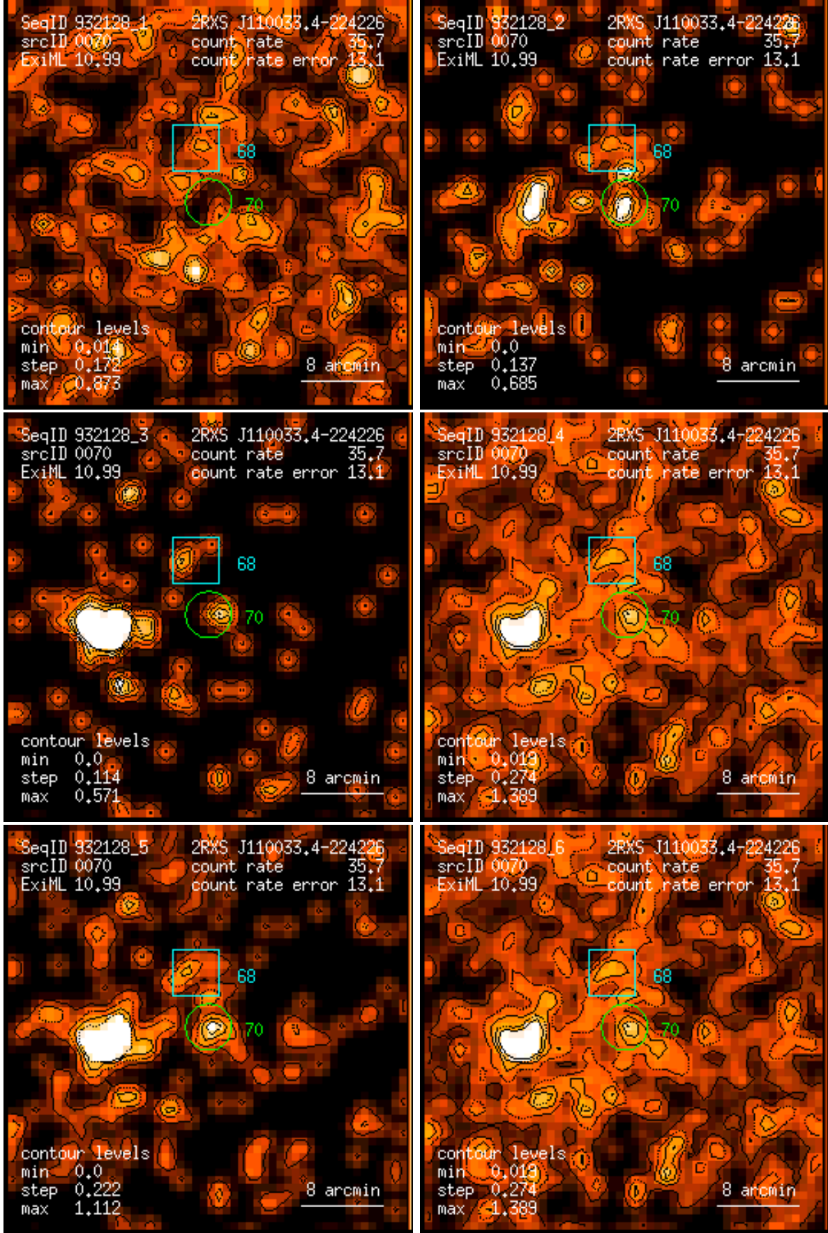
Figure 70: RASS 932128: detection 0070: band rate images, Gaussian filter: (1) PSPC channels 11 – 41, (2) 52 – 90, (3) 91 – 201, (4) 11 – 235, (5) 52 – 201, (6) 11 – 201. Broad band rates in counts/ks. Band rate contour levels in counts/ks/arcmin 2 .
