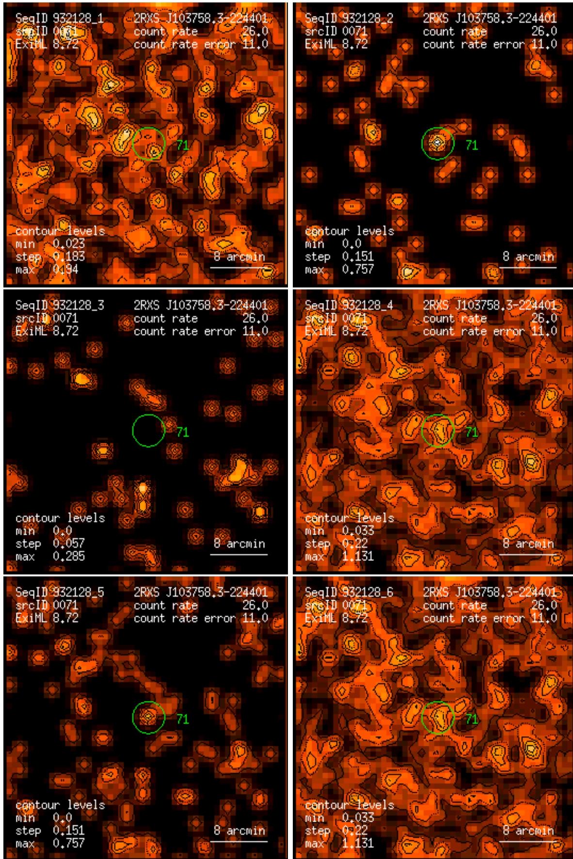
Figure 71: RASS 932128: detection 0071: band rate images, Gaussian filter: (1) PSPC channels 11 – 41, (2) 52 – 90, (3) 91 – 201, (4) 11 – 235, (5) 52 – 201, (6) 11 – 201. Broad band rates in counts/ks. Band rate contour levels in counts/ks/arcmin 2 .
