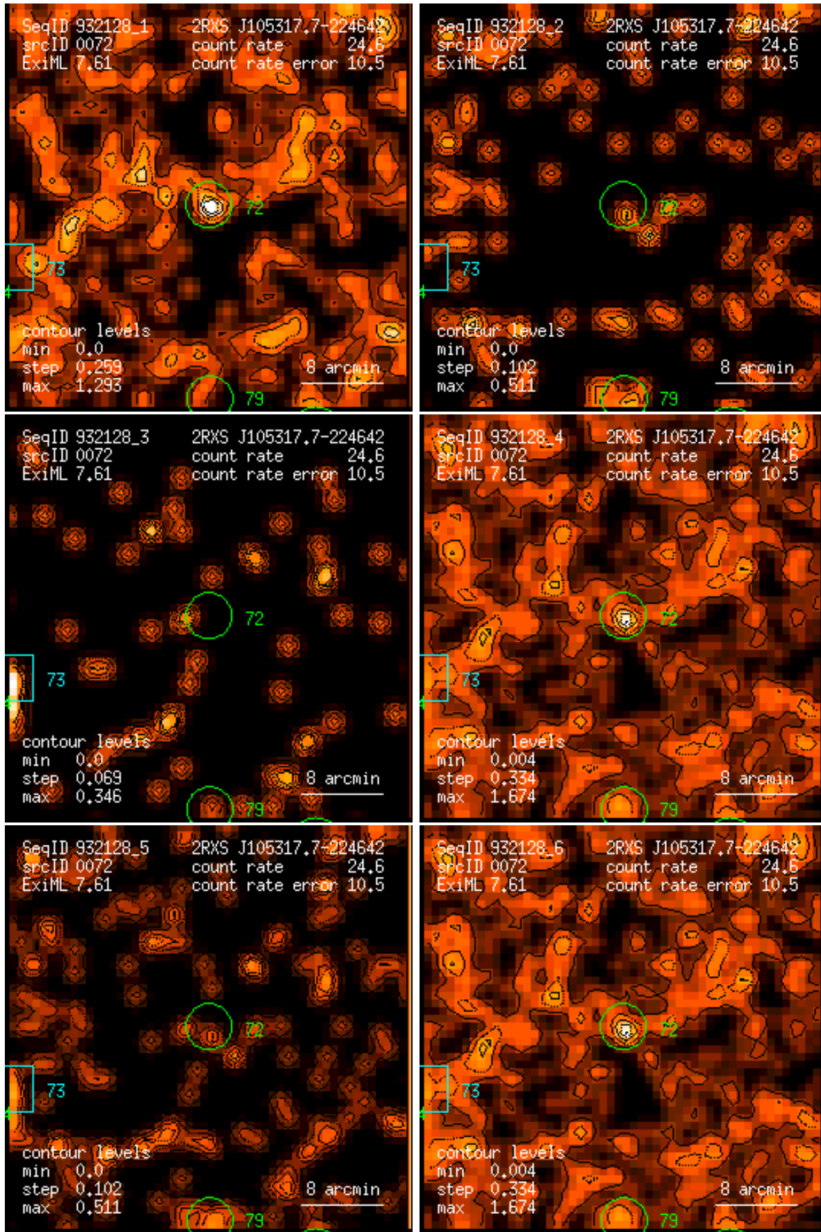
Figure 72: RASS 932128: detection 0072: band rate images, Gaussian filter: (1) PSPC channels 11 – 41, (2) 52 – 90, (3) 91 – 201, (4) 11 – 235, (5) 52 – 201, (6) 11 – 201. Broad band rates in counts/ks. Band rate contour levels in counts/ks/arcmin 2 .
