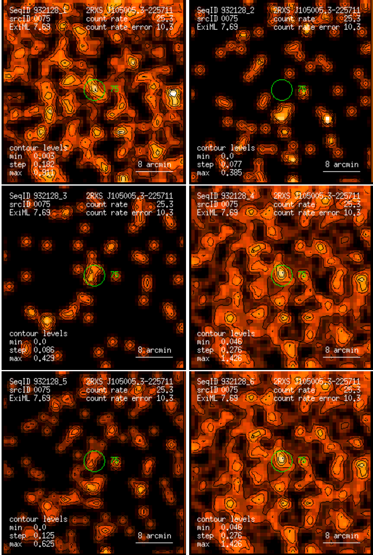
Figure 75: RASS 932128: detection 0075: band rate images, Gaussian filter: (1) PSPC channels 11 – 41, (2) 52 – 90, (3) 91 – 201, (4) 11 – 235, (5) 52 – 201, (6) 11 – 201. Broad band rates in counts/ks. Band rate contour levels in counts/ks/arcmin 2 .
