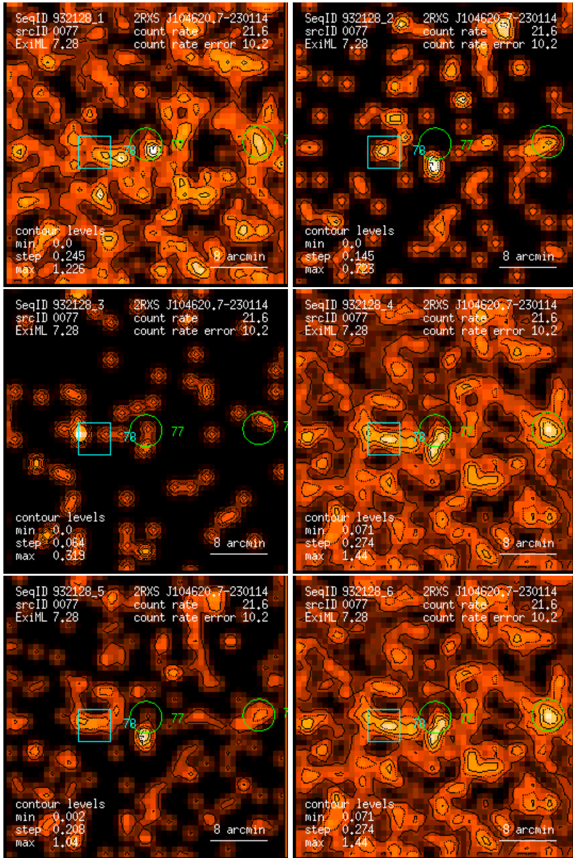
Figure 77: RASS 932128: detection 0077: band rate images, Gaussian filter: (1) PSPC channels 11 – 41, (2) 52 – 90, (3) 91 – 201, (4) 11 – 235, (5) 52 – 201, (6) 11 – 201. Broad band rates in counts/ks. Band rate contour levels in counts/ks/arcmin 2 .
