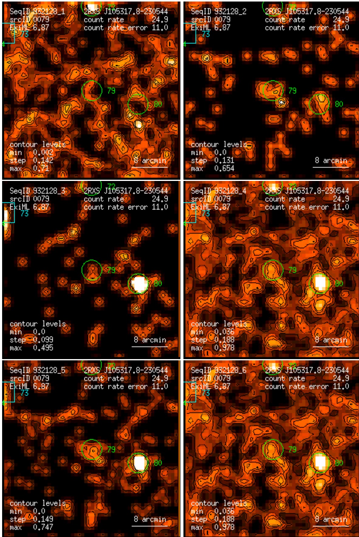
Figure 79: RASS 932128: detection 0079: band rate images, Gaussian filter: (1) PSPC channels 11 – 41, (2) 52 – 90, (3) 91 – 201, (4) 11 – 235, (5) 52 – 201, (6) 11 – 201. Broad band rates in counts/ks. Band rate contour levels in counts/ks/arcmin 2 .
