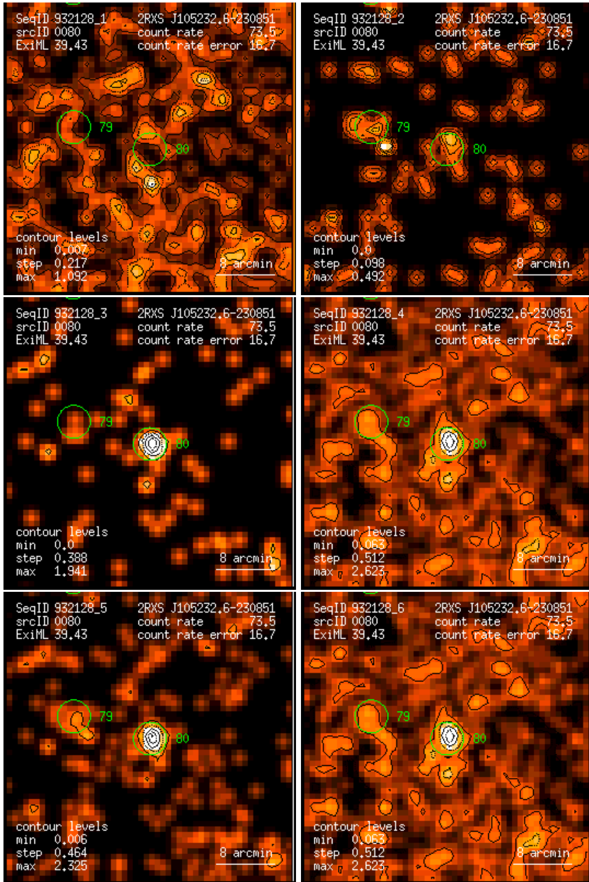
Figure 80: RASS 932128: detection 0080: band rate images, Gaussian filter: (1) PSPC channels 11 – 41, (2) 52 – 90, (3) 91 – 201, (4) 11 – 235, (5) 52 – 201, (6) 11 – 201. Broad band rates in counts/ks. Band rate contour levels in counts/ks/arcmin 2 .
