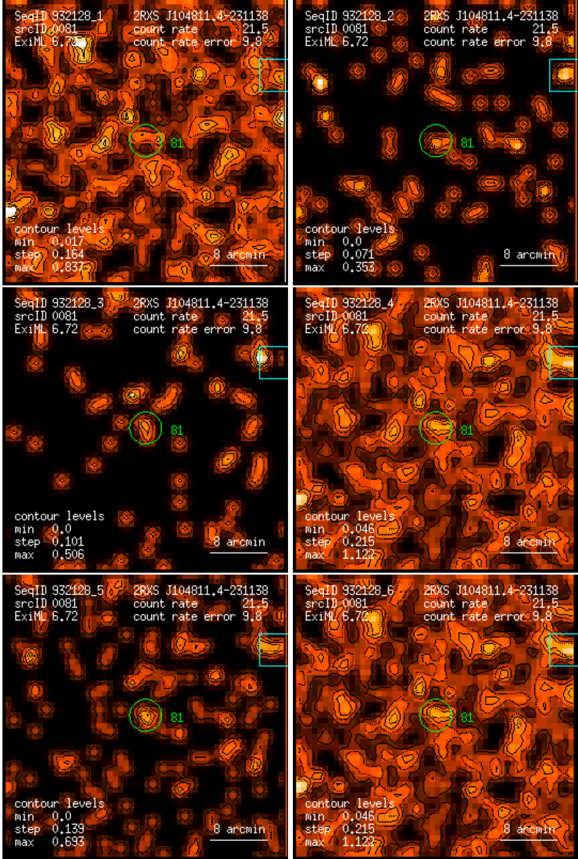
Figure 81: RASS 932128: detection 0081: band rate images, Gaussian filter: (1) PSPC channels 11 – 41, (2) 52 – 90, (3) 91 – 201, (4) 11 – 235, (5) 52 – 201, (6) 11 – 201. Broad band rates in counts/ks. Band rate contour levels in counts/ks/arcmin 2 .
