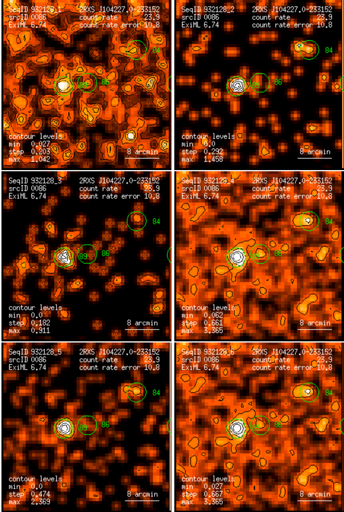
Figure 86: RASS 932128: detection 0086: band rate images, Gaussian filter: (1) PSPC channels 11 – 41, (2) 52 – 90, (3) 91 – 201, (4) 11 – 235, (5) 52 – 201, (6) 11 – 201. Broad band rates in counts/ks. Band rate contour levels in counts/ks/arcmin 2 .
