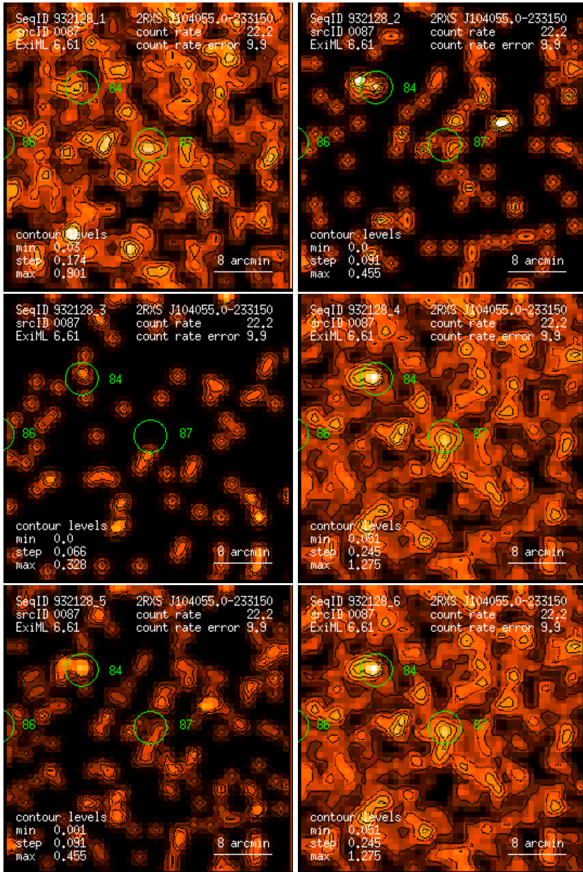
Figure 87: RASS 932128: detection 0087: band rate images, Gaussian filter: (1) PSPC channels 11 – 41, (2) 52 – 90, (3) 91 – 201, (4) 11 – 235, (5) 52 – 201, (6) 11 – 201. Broad band rates in counts/ks. Band rate contour levels in counts/ks/arcmin 2 .
